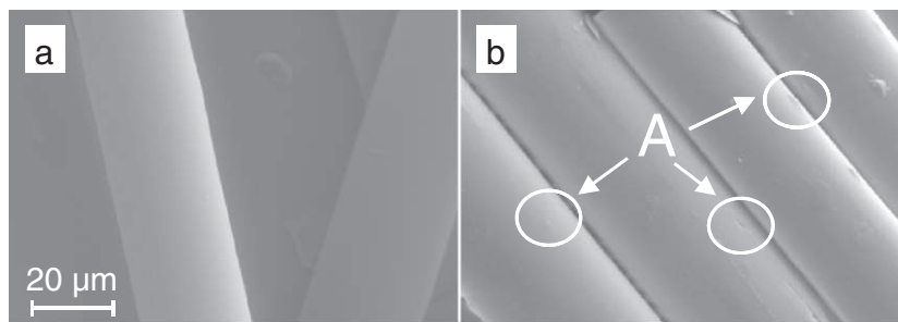
Fig. 3. SEM images of green fibres spun at (a) 280 and (b) 275 °C.
