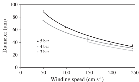
Fig. 4. Variation in diameters with winding speed for green fibres spun at different extrusion pressures (spinning temperature 280 °C, spinneret hole size 300 µm).
