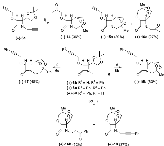
Scheme 4. Gold catalysis for the bis-cycloetherification of bis-alkynic acetonides 6a–d . Synthesis of bridged hybrid \beta -lactam/acetal 14–18 . Conditions: i) 2.5 mol% [AuClPPh 3 ], 2.5 mol% AgOTf, 10 mol% PTSA, 100 mol% H 2 O, CH 2 Cl 2 , sealed tube, 80 °C, 3 h. PTSA = p -Toluenesulfonic acid.
