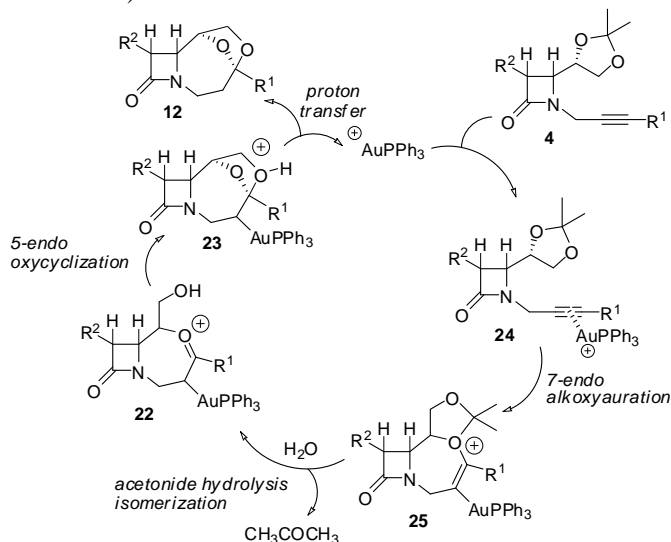
Scheme 6. Mechanistic explanation for the gold-catalyzed bis-oxycyclization of alkynyl acetonides 4 .
