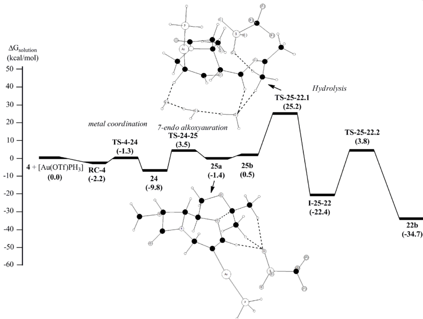
Figure 3. Gibbs energy profile in \text{CH}_2\text{Cl}_2 solution obtained for the gold-catalyzed bis-cyclization of the alkyne acetone 4 at the M06/6-31+G(d) (def2-SVP for Au) theory level. All the energies are referred to the reactants: alkyne acetone ( 4a ) + [\text{Au}(\text{OTf})\text{PH}_3] + water molecules when necessary.
