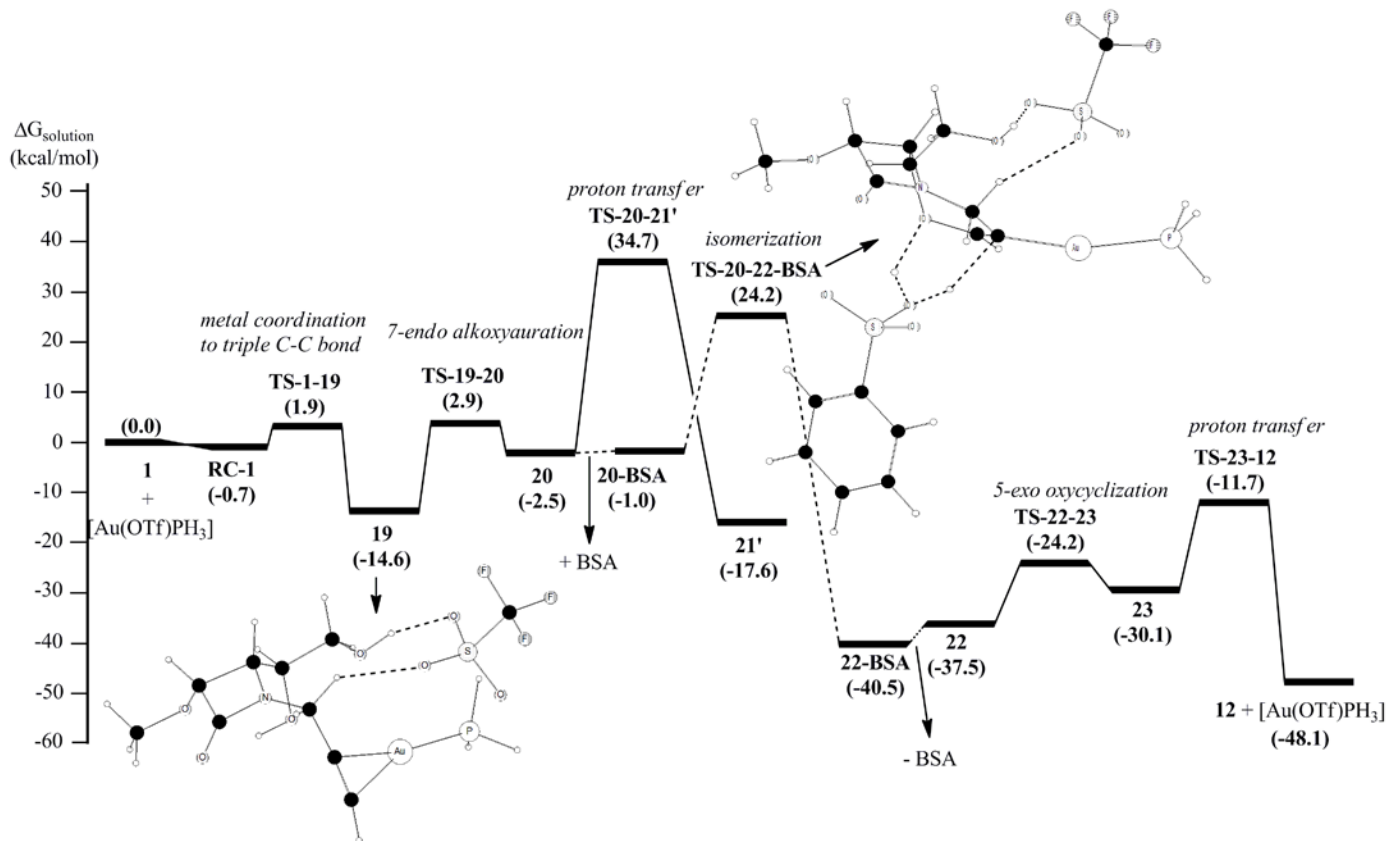
Figure 2. Gibbs energy profile in \text{CH}_2\text{Cl}_2 solution obtained for the gold-catalyzed bis-cyclization of the alkyne 1 at the M06/6-31+G(d) (def2-SVP for Au) theory level. All the energies are referred to the reactants: alkyne 1 , 1,2-diol 1 + [\text{Au}(\text{OTf})\text{PH}_3] + benzenesulfonic acid (BSA).
