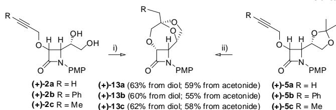
Scheme 3. Gold catalysis for the bis-cycloetherification of alkynic diols 2 and alkynic acetonides 5 . Synthesis of bridged hybrid \beta -lactam/acetal 13 . Conditions: i) 2.5 mol% [AuClPPh 3 ], 2.5 mol% AgOTf, 10 mol% PTSA, CH 2 Cl 2 , RT, 2a : 4 h; 2b : 5 h; 2c : 4 h. ii) 2.5 mol% [AuClPPh 3 ], 2.5 mol% AgOTf, 10 mol% PTSA, 100 mol% H 2 O, CH 2 Cl 2 , sealed tube, 80 °C, 5a : 2 h; 5b : 3 h; 5c : 3 h. PMP = 4-MeOC 6 H 4 . PTSA = p -Toluenesulfonic acid.
