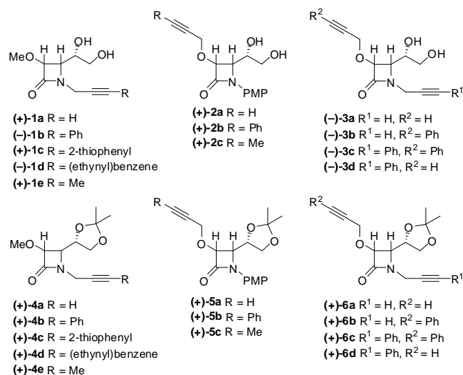
Figure 1. Structures of alkyne diols and alkyne acetonides 1–6 . PMP = 4-MeOC 6 H 4 .
