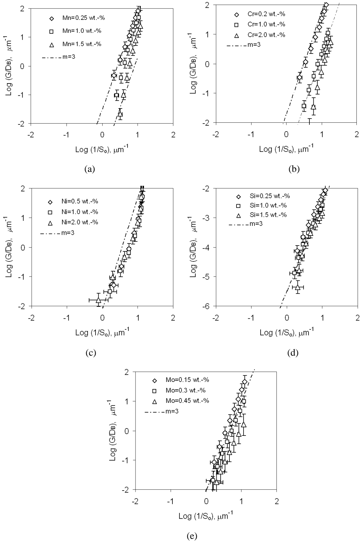
Figure 12. \text{Log}(G_X/D_B^\gamma) vs \text{Log}(1/S_0) plots for (a)Mn, (b)Cr, (c)Ni, (d)Si, and (e)Mo eutectoid steels.
