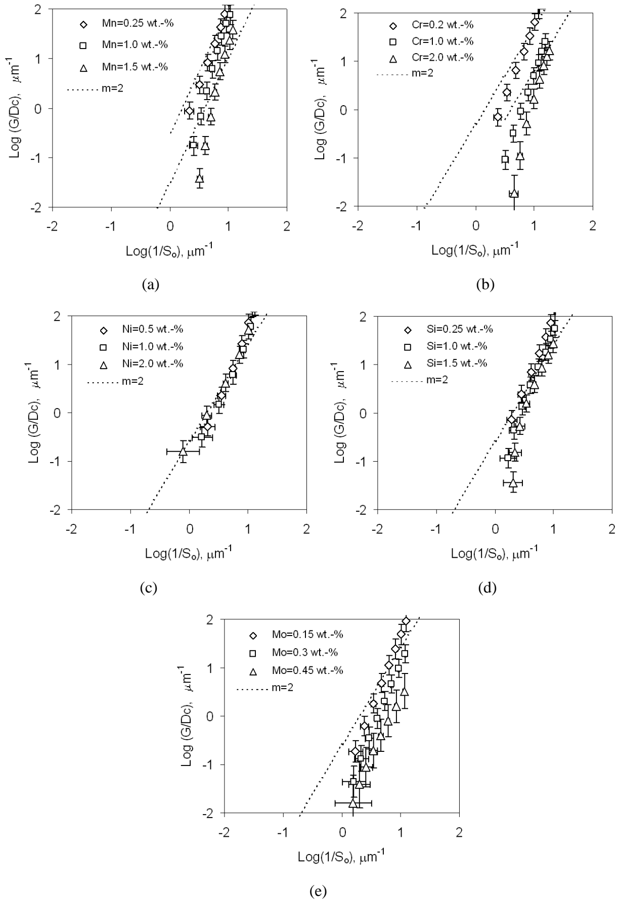
Figure 11. \text{Log}(G_C/D_C^\gamma) vs \text{Log}(1/S_0) plots for (a)Mn, (b)Cr, (c)Ni, (d)Si, and (e)Mo eutectoid steels.
