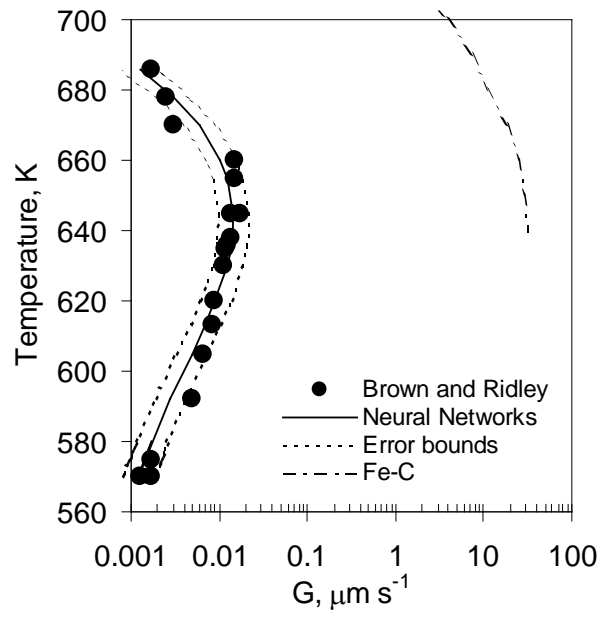
Figure 9. Evolution of pearlite growth rate in a Fe-C-Mn-Cr-Ni-Si-Mo steel
