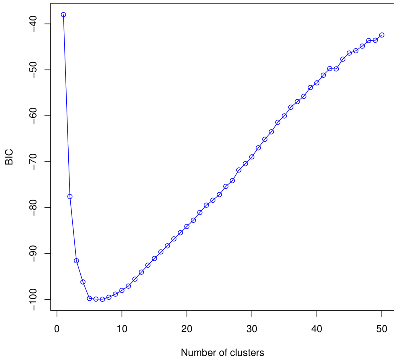
Value of BIC versus number of clusters
