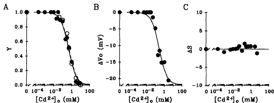
FIGURE 7. Concentration-effect curves of [\text{Cd}^{2+}]_o on G_{AB,\text{max}} , V_o and S (see Materials and Methods, Eq. 2). (A) Ratio ( Y ) between G_{AB,\text{max}} in \text{Cd}^{2+} and in control solution, in 5.4 and 10.8 mM \text{K}^+ (filled and open circles, respectively) fitted to Eq. 3 (continuous and dashed lines, respectively) (see Results). (B) Differences ( \Delta V_o ) between V_o in \text{Cd}^{2+} and in control solution, fitted to Eq. 4 (continuous line) (see Results). (C) Differences ( \Delta S ) between the slope parameter S in \text{Cd}^{2+} and in control solution. All experimental values are means from at least six different preparations.
