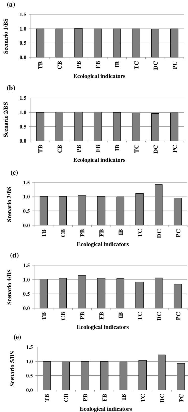
Figure 5. Comparative changes of ecological indicators between baseline simulation (BS) and management scenarios 1 to 5. Ratios less than 1 indicate a decline in biomass or catch over the 45-year simulation (from 1975 to 2020). TB = Total biomass, CB = commercial species biomass, PB = predator species biomass, FB = Fish biomass, IB = Invertebrates (except plankton) biomass, TC = Total catch, DC = Demersal catch, PC = Pelagic catch.
