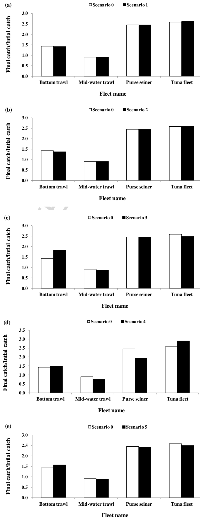
Figure 6. Catch changes by fleet for the baseline simulation (scenario 0) and management scenarios 1 to 5 at the end of the 45-year simulation (year 2020). Ratios lower than 1 indicate a decline catch over the 45-year simulation (from 1975 to 2020).
