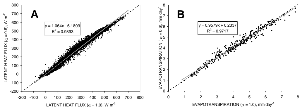
7 Fig. 7. Correlations of half hourly values of latent heat flux (A) for \alpha=0.6 versus 8 \alpha=1.0 and daily values of evapotranspiration (B) for \alpha=0.6 versus \alpha=1.0 using 9 all the data from 2007 and 2008. The solid lines represents the linear regression 10 obtained in both cases, the dashed lines represents the straight line y=x .
