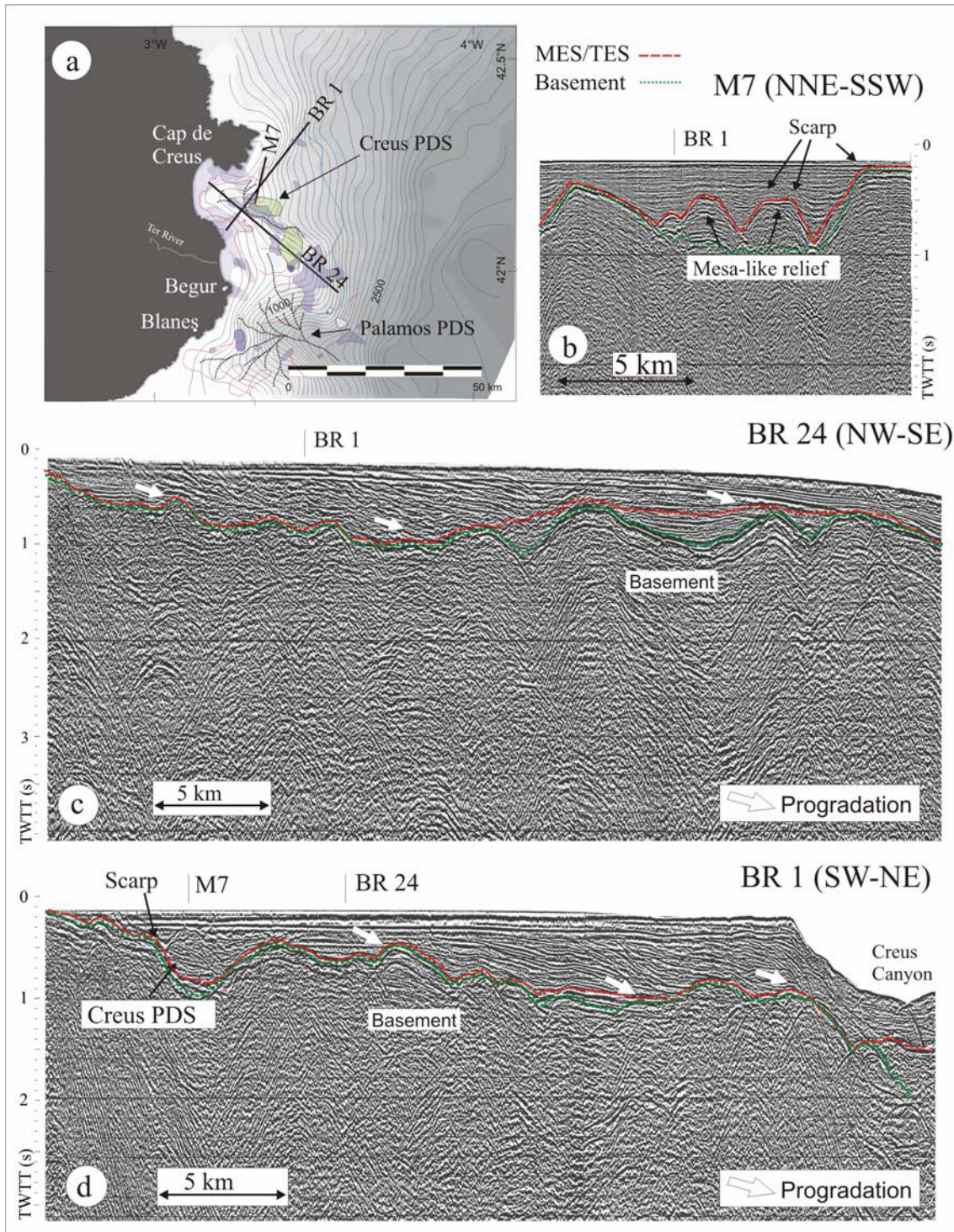
Figure 6. The Creus domain is the northernmost domain of the study area, limited to the south by the Palamós paleo-drainage system (PDS). a) Bathymetry of the MES/TES and location of the seismic profiles (see legend in Figure 5). b) to d) Seismic profiles showing the MES/TES, which coincides in many cases with the basement. White arrows mark the progradation of the Plio-Quaternary sediments on the MES/TES. Figure 6d shows the mesa-like reliefs on the Creus PDS.
