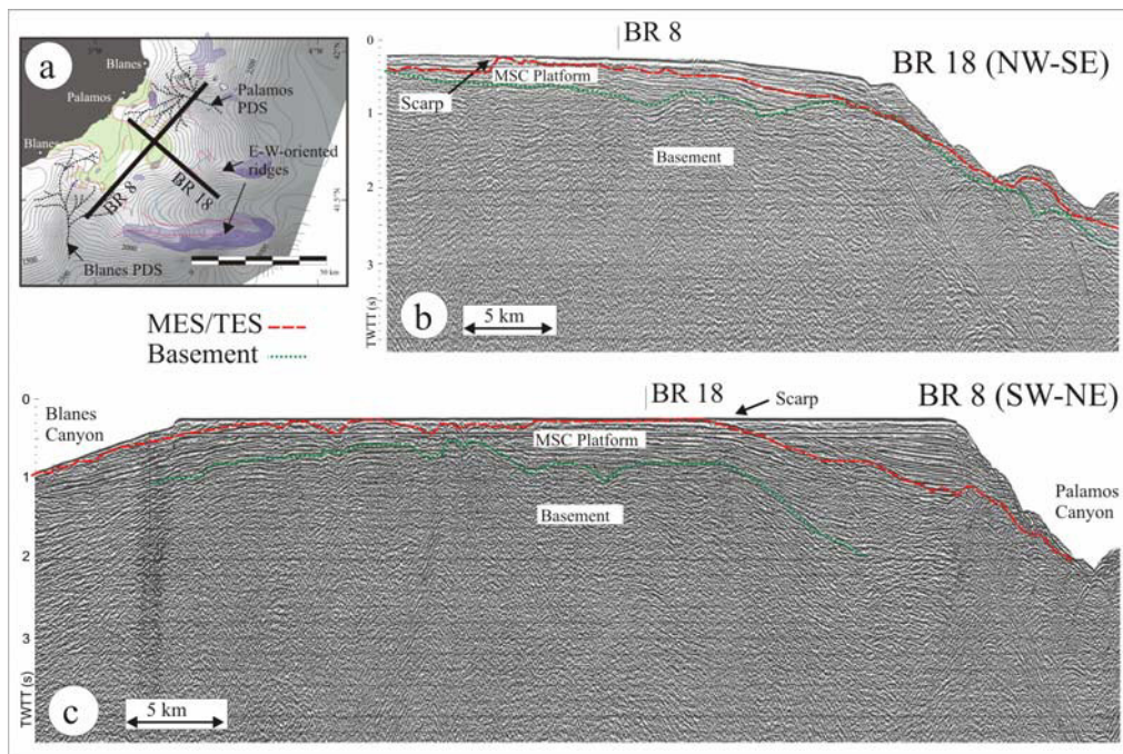
Figure 7. The Girona domain is limited by the Palamós PDS to the north and by the Blanes PDS to the south. a) Bathymetry of the MES/TES and location of the seismic profiles (see legend in Figure 5). b) and c) Seismic profiles showing the MES/TES and the basement. This domain is characterized by a wide and flat MCS platform.
