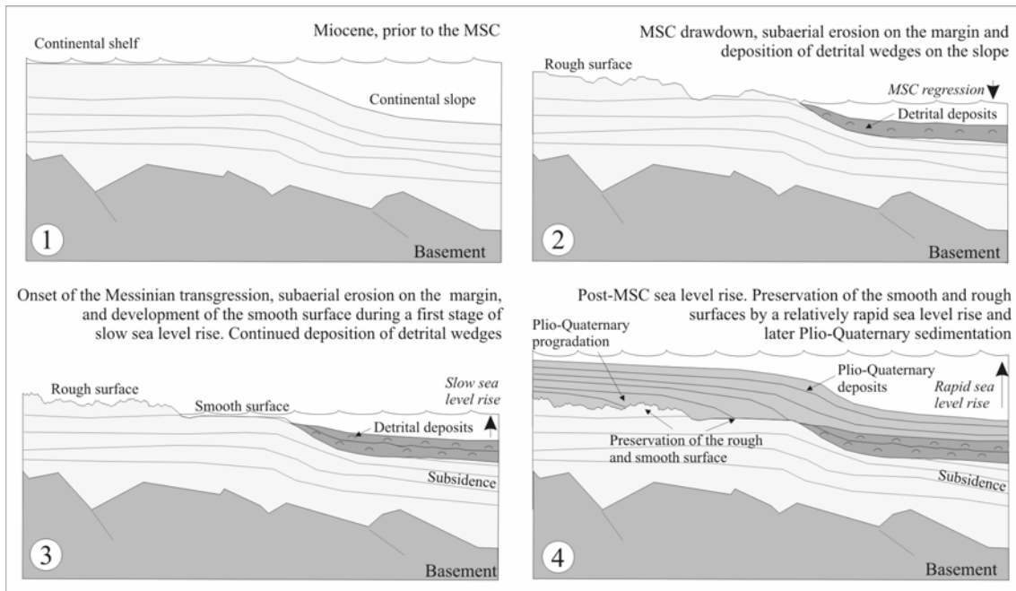
Figure 12. Schematic diagram of the sea level changes during the MSC and the resulting rough and smooth erosion surfaces and deposits on the continental shelf and slope.
