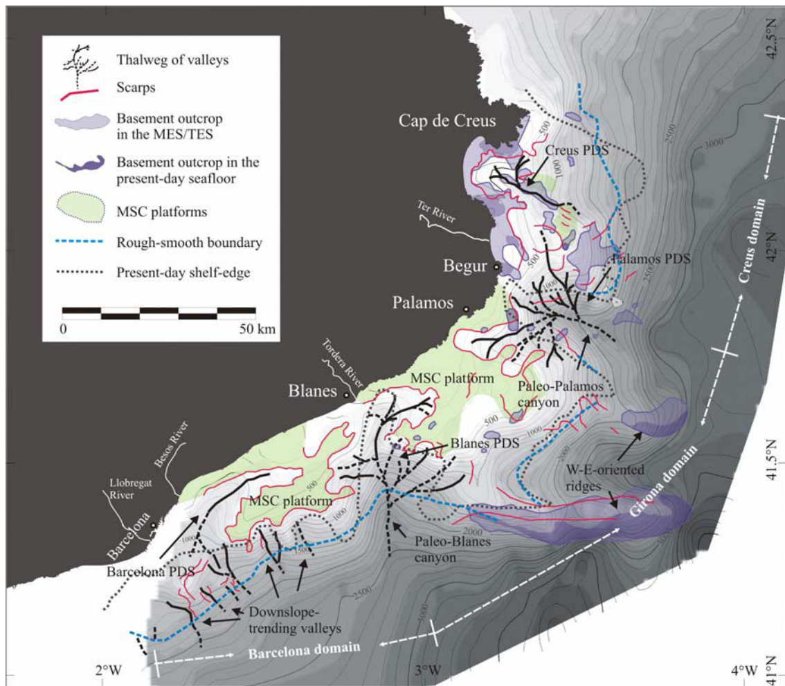
Figure 5. MES/TES isochrone (greyscale) and main morphological features identified on the Catalan margin. The area has been divided into the Creus, Girona and Barcelona domains (from north to south) based on the characteristics of the MES/TES. PDS: Paleo-drainage System.
