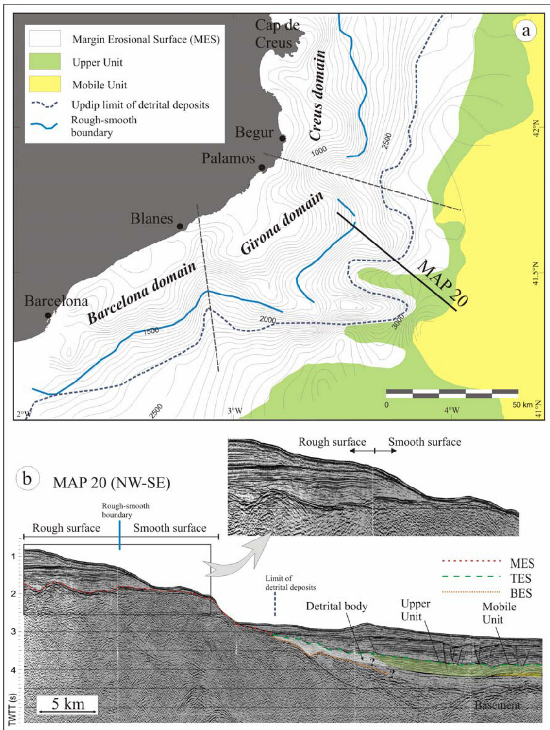
Figure 10. MSC erosional and depositional features. a) Map showing the rough-smooth boundary for the MES/TES, the upper limit of the detrital deposits and the distribution of the Upper and Mobile Units. b) Seismic profile showing the Messinian erosional surfaces (MES, TES, BES) and depositional units in the Valencia Basin.
