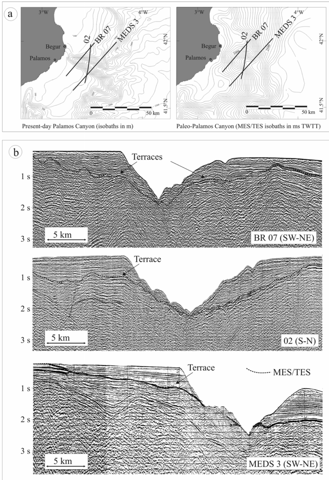
Figure 9. The Palamós present-day- and paleo-canyon. a) Bathymetry of the present-day (isobaths in m) and paleo-canyon (isobaths in ms). b) Seismic profiles showing the present-day and paleo-transversal profile.
