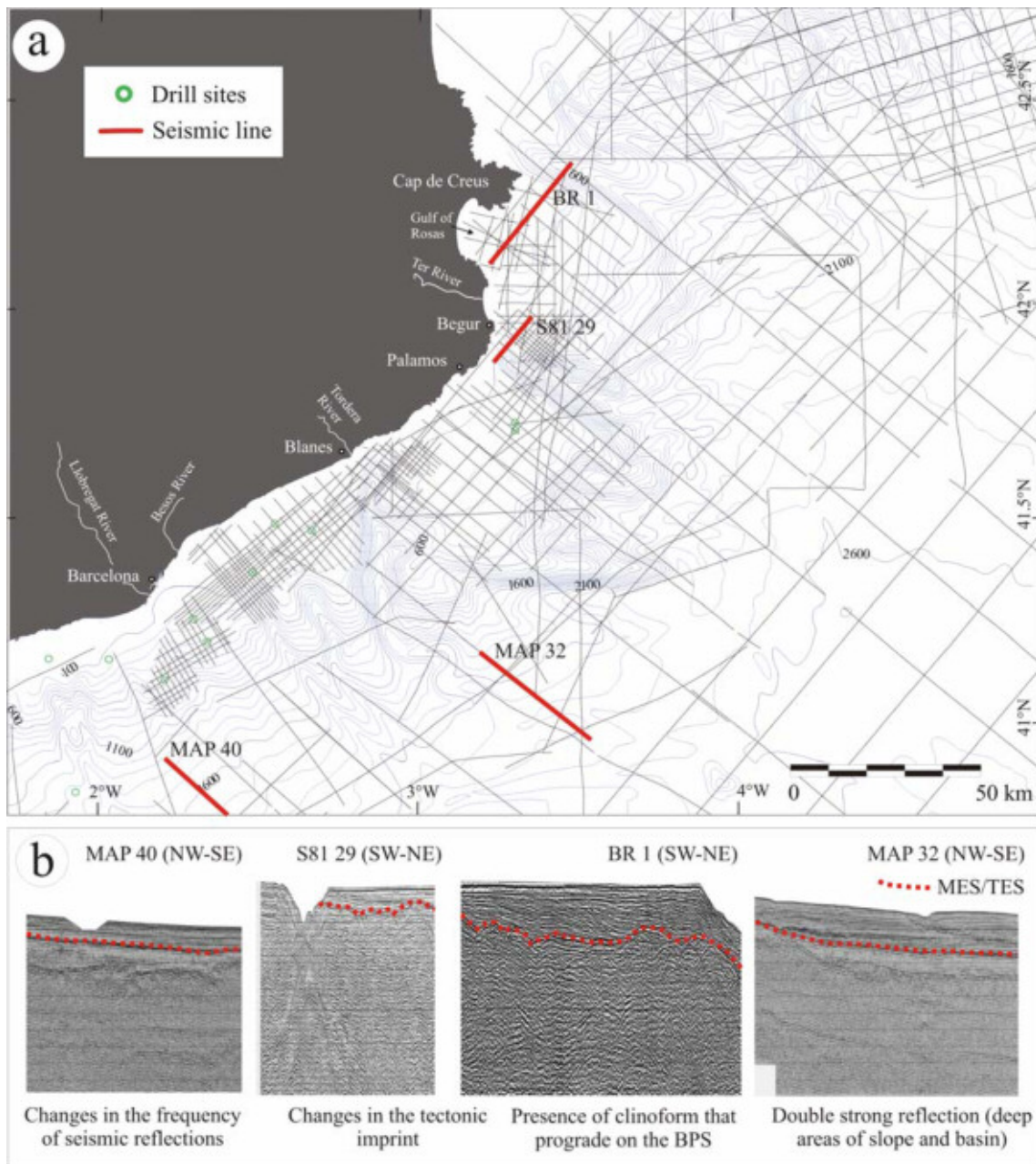
Figure 4. Methodology and dataset. a) Seismic profiles database analysed in this work, including information from the SIGEOF database (IGME) and data from research cruises. b) Examples of seismic profiles showing the criteria for the identification of the MES/TES.
