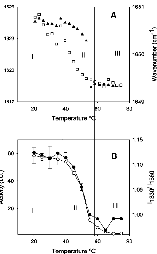
FIGURE 3 Thermal profile of MAT. (A) Traces corresponding to the IR 1652 cm -1 band ( \square ) assigned to \alpha -helix and 1624 cm -1 band ( \blacktriangle ) corresponding to the oligomer interactions in MAT measured in D 2 O buffer. (B) Profiles corresponding to protein activity ( \bullet ) and intrinsic fluorescence ( \circ ).
