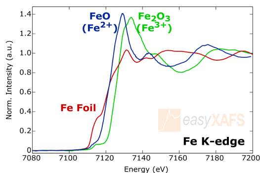
Transition metal XANES is fast, simple, and has synchrotron-grade energy resolution.
