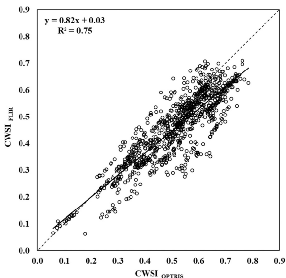
Fig. 12. Relationship between the crop water stress index (CWSI) calculated with FLIR One Pro and Optris Xi 400 sensors for all treatments and years.
