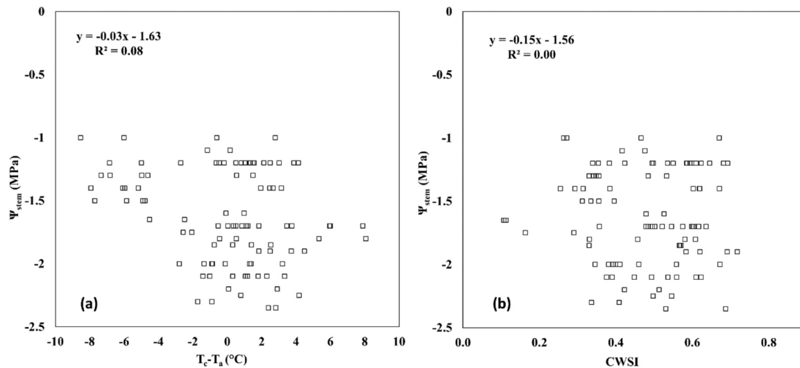
Fig. 15. Relationship between midday stem water potential ( \Psi_{stem} ) and the difference between canopy ( T_c ) and air temperature ( T_a ) (a) and crop water stress index (CWSI) (b) determined for all treatments and years.
