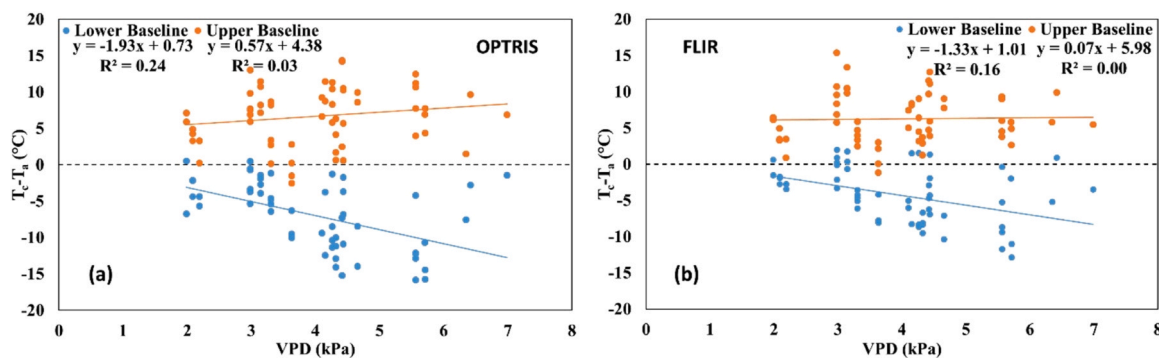
Fig. 9. Difference between canopy temperature ( T_c ) obtained from (a) Optris Xi 400 and (b) FLIR One Pro; and air temperature ( T_a ) as a function of observed Vapor Pressure Deficit (VPD) for all treatments and years.
