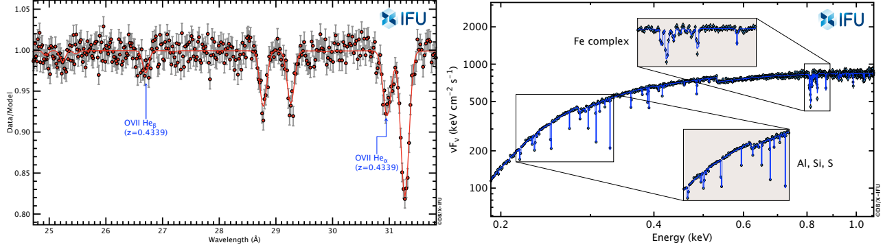
Figure 2. Left) Simulated X-IFU spectrum of an intervening absorber in the Warm-Hot Intergalactic Medium at z=0.4339 . The plot shows the ratio of the X-IFU data of the blazar 1ES 1553+113 with the local best-fitting continuum model, to highlight the two OVII He- \alpha and He- \beta absorption lines. The simulation is performed using the best fitting parameters derived from the long XMM-Newton RGS observations. 21 Right) A simulated X-IFU X-ray spectrum of a medium bright (fluence = 0.4 \times 10^{-6} erg \text{cm}^{-2} ) Gamma-Ray Burst (GRB) afterglow at z = 7 , characterized by deep narrow resonant lines of Fe, Si, S, Ar, Mg, from the gas in the environment of the GRB. An effective intrinsic column density of 2 \times 10^{22} \text{cm}^{-2} has been adopted.
