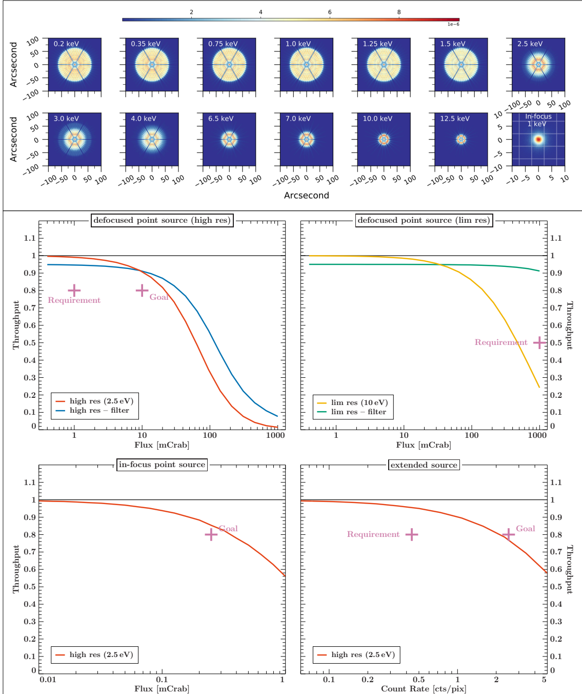
Figure 22. Top: The defocused PSF of the Athena optics at 13 energies as seen by X-IFU. 76 The bottom rightmost panel shows the in-focus PSF at 1 keV (Half Energy Width = 5'' ), for comparison. The grid in this panel shows the X-IFU pixels. We note that the in-focus PSF is shown on a 20'' \times 20'' image while the defocused PSF is shown on a 200'' \times 200'' image. The full field of view of the X-IFU is of the order of 300'' (equivalent diameter). Bottom: Summary of the throughput performance for all the observing cases specified in the X-IFU URD. Requirements and goals are shown with crosses. Top left: High resolution observation of a defocused point source. Top right: Limited resolution (10 eV) observation of a defocused point source (for the filter configuration, the plot includes the 5 % loss due to the limited transmission of the beryllium filter in the 5 to 8 keV band of interest). Bottom left: High resolution observation of a focused point source. Bottom right: High resolution observation of an extended source.
