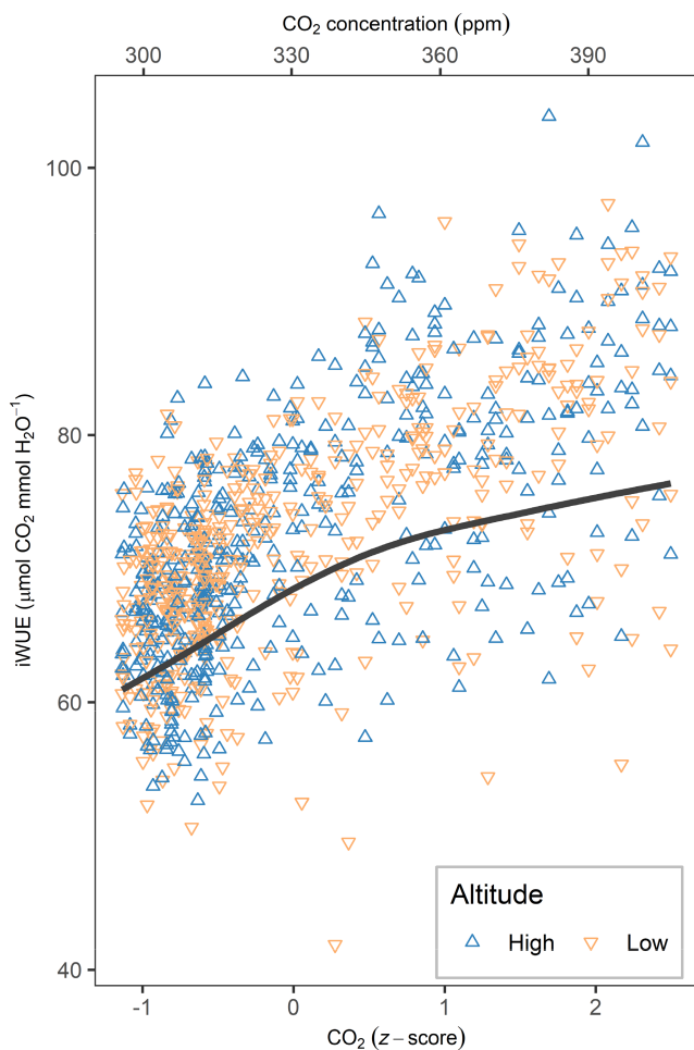
FIGURE 3 Effect of CO 2 on intrinsic water use efficiency (iWUE). Triangles depict observations by altitude (blue upper looking upward, high altitude, orange looking downward, low altitude) and the solid line is the iWUE prediction from the generalized additive mixed model where CO 2 is expressed as a smoothing function of with 2.283 estimated degrees of freedom. Altitude did not show significant effect in this relationship.
