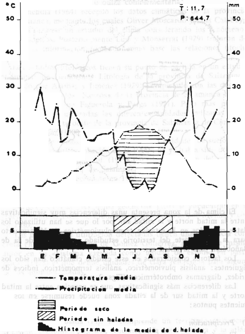
Fig. 2. — DIAGRAMA CLIMATICO (1956 - 1973)
