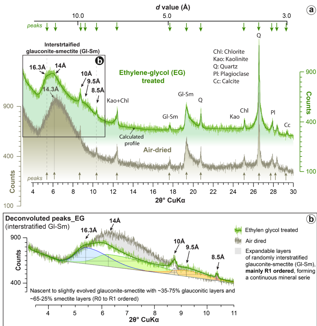
Figure 5. (a) Representative powder XRD diagrams of air-dried and ethylene-glycol treated glaucony concentrates from core 5, with notation of d value. Note the strong reflection at 14.3\text{\AA} that shifted to 16.3\text{\AA} after ethylene-glycol treatment, characteristic of smectite-rich interstratified glauconite-smectite. (b) Deconvoluted d_{001} peak and overlapping peaks after ethylene-glycol-treated glaucony. The strong response to ethylene-glycol treatment is indicative of expandable smectite layers. Deconvoluted peaks correspond mostly to R1, with minor presence of R0, mica/smectite.
