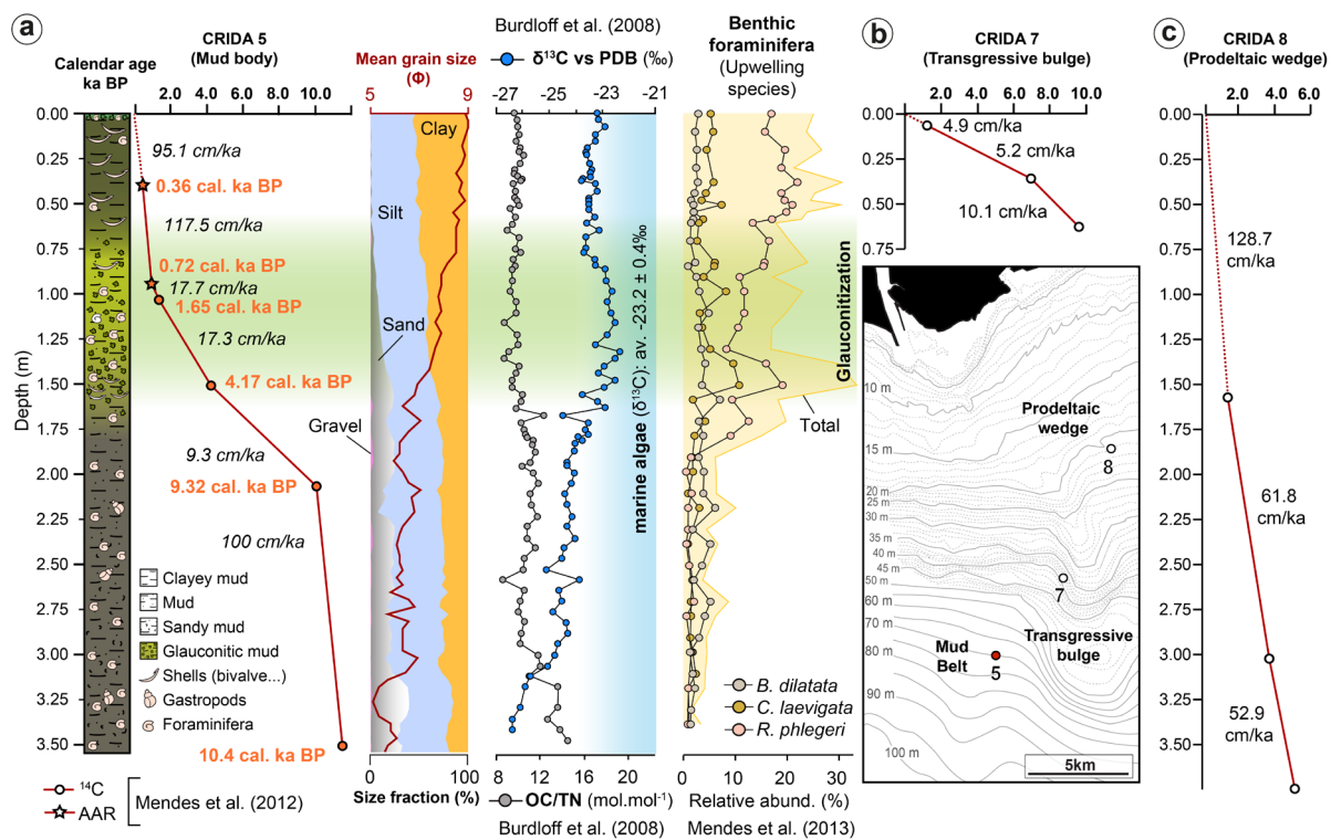
Figure 2. Contrasting sedimentary environments on the continental shelf off the Guadiana River. (a) Core 5 (middle shelf mud belt). (b) Core 7 (proximal zone of a transgressive sandy deposit). (c) Core 8 (inner shelf prodeltaic wedge). Age models based on calibrated ages and sedimentation rates are included (adapted from Mendes et al. [29]). In (a), bottom-up variation in size fractions and mean grain size [29], \delta^{13}\text{C} and OC/TN concentrations (<63 \mu\text{m} fraction of carbonate-free samples; [47]), and relative abundance (%) of benthic foraminiferal species associated with upwelling conditions [55] are also indicated. The glauconitization process is highlighted.
