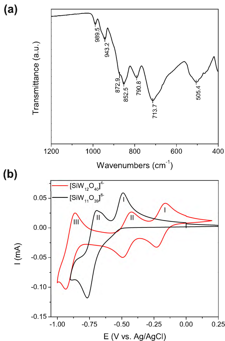
Figure 1. POM characterization. (a) Infrared spectra of the solid POM (indexed peaks found on Table S1). (b) Cyclic voltammetry of the lacunary [SiW 11 O 39 ] 8- (POM) anion compared with the commercial parent [SiW 12 O 40 ] 4- anion in 1 M sodium acetate buffer (pH 4.7); scan rate: 50 mV/s, POM concentration: 5 mM.
