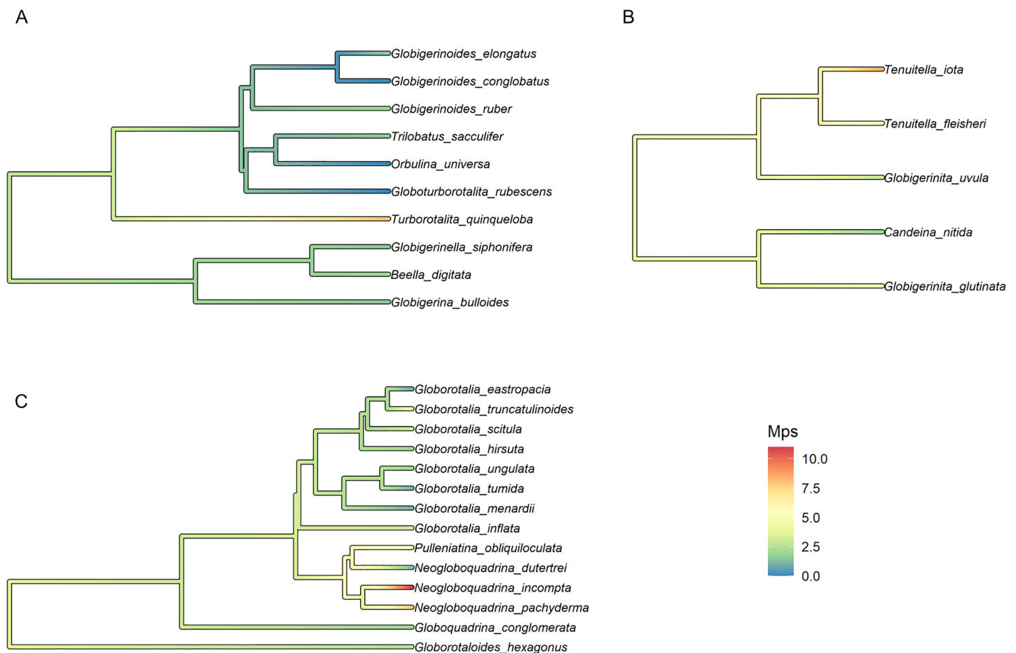
Figure 3 Ancestral state reconstruction of the median number of polymorphic sites. Ancestral state reconstruction of the median number of polymorphic sites (Mps) in (A) Spinose, (B) Microperforate and (C) Non-Spinose phylogenetic trees. Full-size DOI: 10.7717/peerj.15255/fig-3
