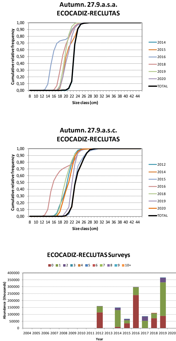
Figure 3.2.23. ECOCADIZ-RECLUTAS Autumn acoustic-trawl survey series. Upper and middle panels: cumulative size frequencies for chub mackerel. Total refers to pooled data for the available time-series (2012–2020). Bottom panel: age structure of the estimated population in the surveyed area (27.9.a.s) in 2012–2019 surveys. Age structure in 2012–2018 surveys estimated by applying IEO’s age–length keys from 27.8.c–27.9.a.n subareas (source: Ramos and Carrera presentation during the WK; abstract without figures available in Annex 4).
