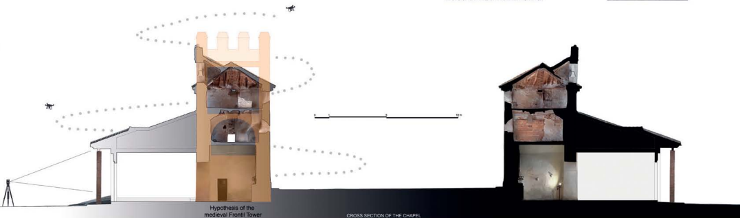
CROSS SECTION OF THE CHAPEL
