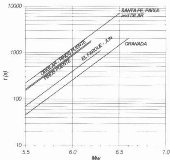
Figure 2. Return period ( t ) as a function of the moment magnitude ( M_w ) for the faults in the Granada basin where a smaller value of t corresponds to a higher slip rate. The curves have been plotted up to the maximum magnitude that the fault is able to produce.
