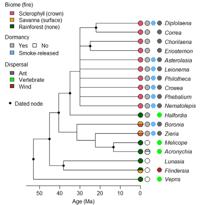
Fig. 8. Dated molecular phylogeny of the main genera in Rutaceae, subfamily Amyridoideae, that occur in Oceania (plus Vepris in Africa). For each genus, symbols indicate the current biome (sclerophyll woodlands and shrublands, savanna, rainforest) and associated fire regime (crown, surface, or no fires), seed dormancy, experimental evidence for smoke-sensitive germination (at least for those species examined), and dispersal mode (vertebrate dispersal refers mainly to birds, but in some cases includes mammals, such as primates dispersing Vepris ). Missing symbols indicate missing information. Note that it is unlikely that smoke-germination experiments have been conducted on rainforest species as it is not fireprone; nevertheless, many of these are non-dormant. Symbols with two colours indicate species inhabiting two habitats or with uncertainty. Undated nodes are arbitrarily located at the midpoint of the stem. Despite some phylogenetic uncertainties, it is clear that rainforest habitats and vertebrate dispersal are ancestral, while crown-fire habitats and ant dispersal are derived. Phylogeny from Paetzold et al. (2018) and Bayly et al. (2013); smoke-released dormancy and ant dispersal from Data S1; other dispersal modes from Lieberman et al. (1979), Bayly et al. (2013), Gould & Gabriel (2015), Appelhans et al. (2018) and Paetzold et al. (2018).
