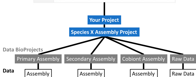
Fig. 2. Recommended EBP INSDC assembly BioProject submission structure. Alternatives on this theme could include maternal assembly and paternal assembly at the DataBioProject levels, when complete genome assemblies are generated for both haplotypes of a diploid sexually reproducing species. "Your Project" represents a project sequencing multiple genomes, such as the VGP or DTOL.
