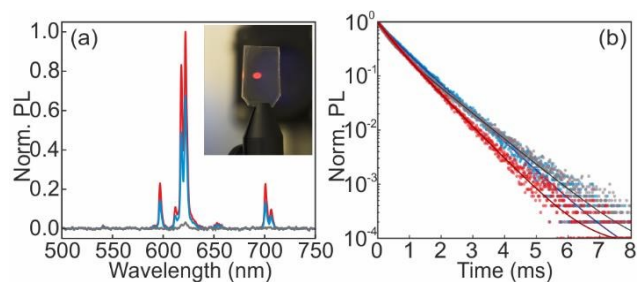
Fig. 3: (a) Normalized photoluminescence (PL) of \text{GdVO}_4:\text{Eu}^{3+} films as-deposited (grey), and annealed at 1000^\circ\text{C} in a conventional oven (red), or using RTA (blue). Inset shows the red emission of the film annealed at 1000^\circ\text{C} with RTA upon excitation with a 285 nm LED. (b) Time-dependent PL of the same films. Fitting curves to a double exponential model are also shown as black lines.
