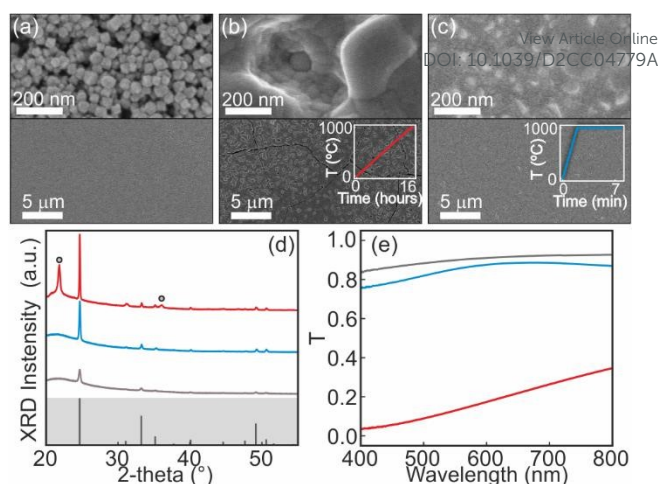
Fig. 2: (a–c) Scanning electron micrographs of the top view of \text{GdVO}_4:\text{Eu}^{3+} nanophosphor films as-deposited (a), and annealed at 1000 °C in a conventional oven (b) or using RTA (c). Insets show time profiles of the thermal processing. (d) X-ray diffraction patterns of samples as-deposited (grey), annealed at 1000 °C in a conventional oven (red) and 1000 °C with RTA (blue). Diffraction pattern of standard PDF-86-0996 (ICDD 2014) is also shown as grey lines for comparison. Circles highlight reflections associated to cristobalite structure. (e) Zeroth-order transmittance for light incident in a close-to-normal direction for as-deposited nanophosphor films (grey), and films annealed at 1000 °C in a conventional oven (red) or using RTA (blue).
