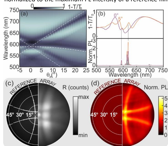
Fig. 4: (a) Angular dependence of the extinction spectra measured from the nanophosphor film coated with the plasmonic sticker. (b) Extinction spectra (top) at 0^\circ (purple) and 5^\circ (orange). Rayleigh anomalies (RAs) of (\pm 1, 0) and (0, \pm 1) diffracted orders are also shown as dashed white lines. Photoluminescence (PL) intensity spectra (bottom) collected from the nanophosphor film coated with the plasmonic sticker at 0^\circ (purple) and 5^\circ (orange). PL of a reference film is also shown for comparison (shaded grey curve). All spectra are normalized to the maximum intensity of the reference. (c–d) Fourier image of the reflectivity (c) and PL (d) at 620 nm of the nanophosphor film coated with the plasmonic sticker (right semicircle) and that of the reference film (left semicircle). RAs of (\pm 1, 0) diffracted orders are also shown as dashed white lines. Values are normalized to the maximum intensity measured for the reference.
