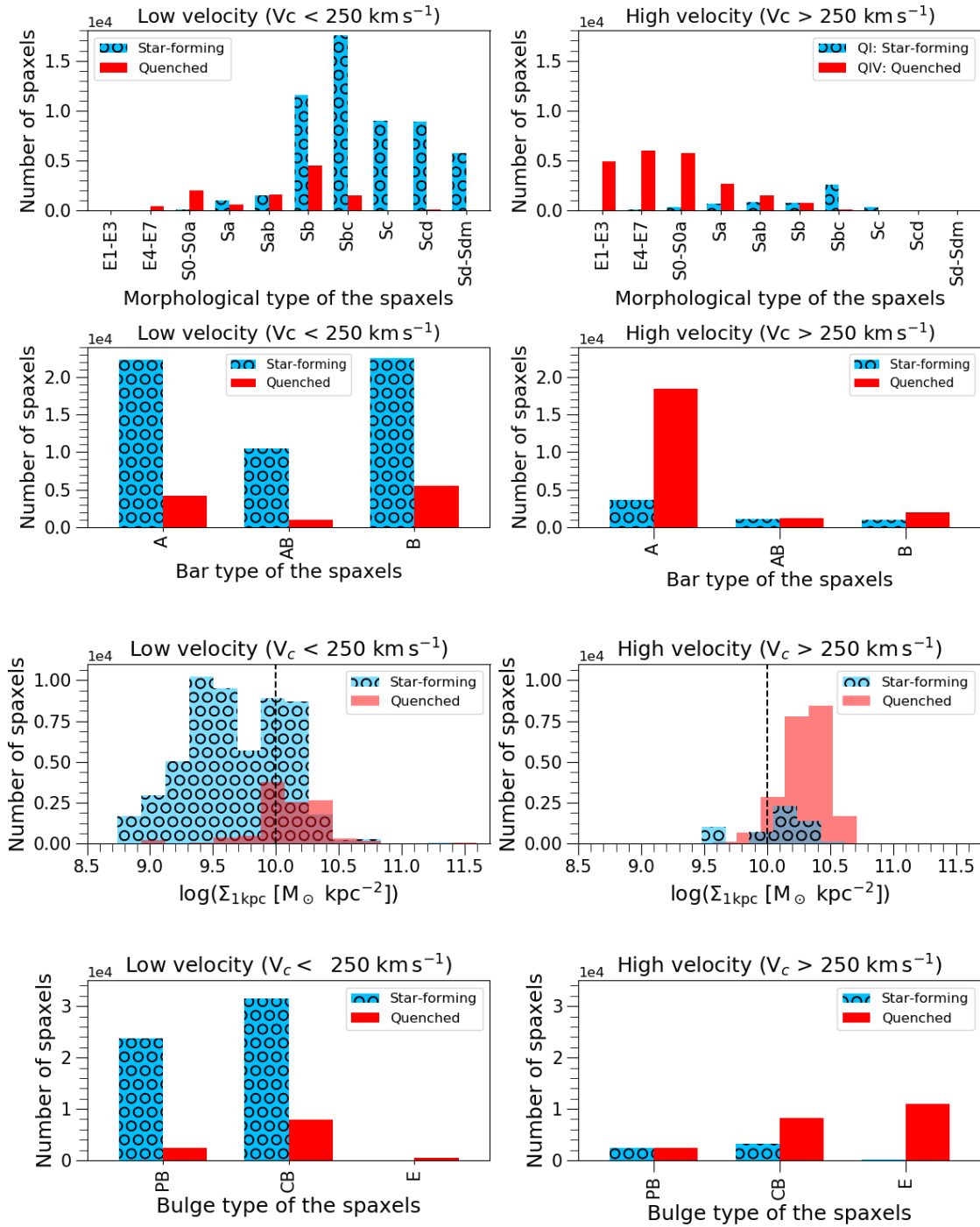
Fig. 5. Spaxel distribution of W_{\text{H}\alpha} - V_c relation across properties of the host galaxies. The first and second row panels correspond to the morphological and bar-type (A: no bar, B: bar, and AB: unsure bar) classifications of the galaxies from Walcher et al. (2014), respectively. The third row panels explore the central stellar mass surface density ( \Sigma_{1\text{kpc}} ) of the host galaxies, following Cheung et al. (2012). The fourth row panels relate to the bulge type of the host galaxies, according to the method described in Luo et al. (2020, PB: pseudo bulge, CB: classical bulge, and E: ellipticals). The left column panels explore the statistics of the spaxels for low velocities ( V_c < 250\text{ km s}^{-1} ), while the right panels correspond to the high velocities ( V_c > 250\text{ km s}^{-1} ). The different colours and symbols of the bars distinguish star-forming (blue with black circle) and quenched (red with no symbol) regions of the galaxies. The dashed horizontal lines at \Sigma_{1\text{kpc}} = 10^{10} M_{\odot} \text{ kpc}^{-2} are drawn to guide the eye. See more details in Sect. 3.2.
