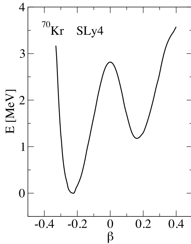
Figure A.6. Potential energy curve for ^{70}\text{Kr} obtained from constrained HF + BCS calculations with the Skyrme force SLy4.
