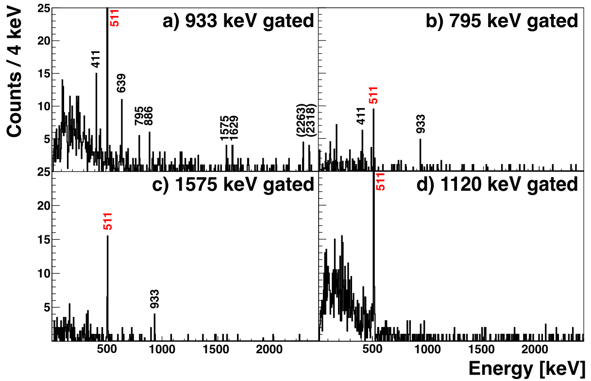
Figure A.5. Energy spectra of the \beta -delayed \gamma -rays in coincidence with the a) 933 keV \gamma -transition; b) 795 keV \gamma -transition; c) 1575 keV \gamma -transition; d) 1120 keV \gamma -transition.
