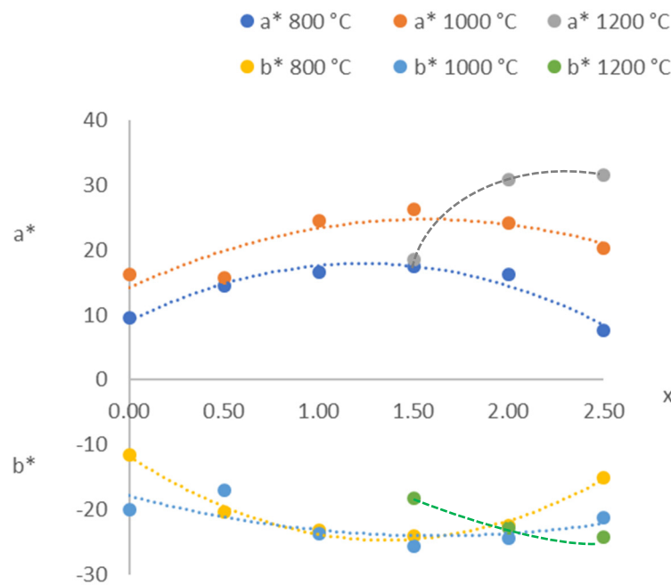
Figure 7. CIE L*a*b* from the Mg x Co 3-x P 2 O 8 compositions fired at 800, 1000 and 1200 °C.
