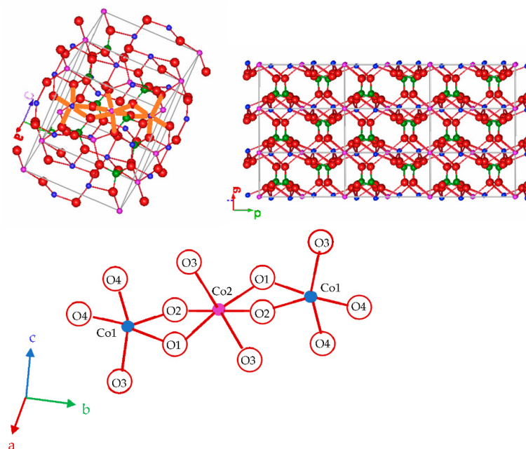
Figure 1. Stable \text{Co}_3\text{P}_2\text{O}_8 structure. The colour scheme to represent the atoms is O (-II): red, P(V): green, Co(II): blue with CN = 5, and lilac with CN = 6.
