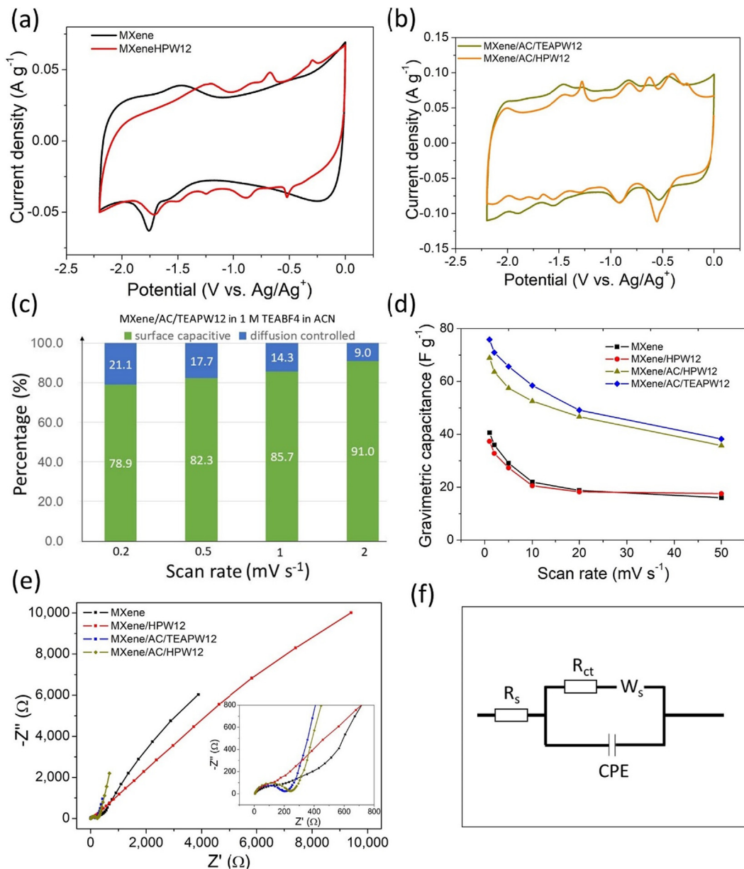
Fig. 6. (a) Cyclic voltammograms of MXene and MXeneHPW12 at 1 mV s -1 in 1 M TEABF4 acetonitrile. (b) Cyclic voltammograms of MXene/AC/HPW12 and MXene/AC/TEAPW12 at 1 mV s -1 in 1 M TEABF4 acetonitrile. (c) Surface capacitive contribution and diffusion-controlled contribution at various scan rates. (d) Gravimetric capacitance of MXene, MXene/HPW12, MXene/AC/HPW12 and MXene/AC/TEAPW12 at various scan rates. (e) Electrochemical impedance spectra of MXene, MXene/HPW12, MXene/AC/HPW12 and MXene/AC/TEAPW12. (f) Equivalent circuit for fitting impedance spectra.
