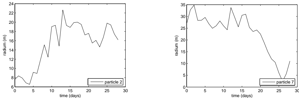
Fig. 2 – Temporal evolution of the radial position for two particles at 100 m depth, initially located at different distances from the eddy center.
