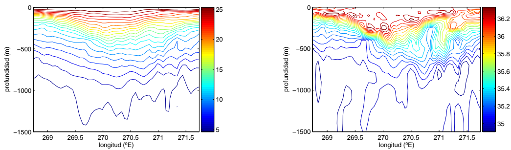
Fig. 1 – Vertical section of temperature (left) and salinity (right) 10 days after the eddy’s formation.
