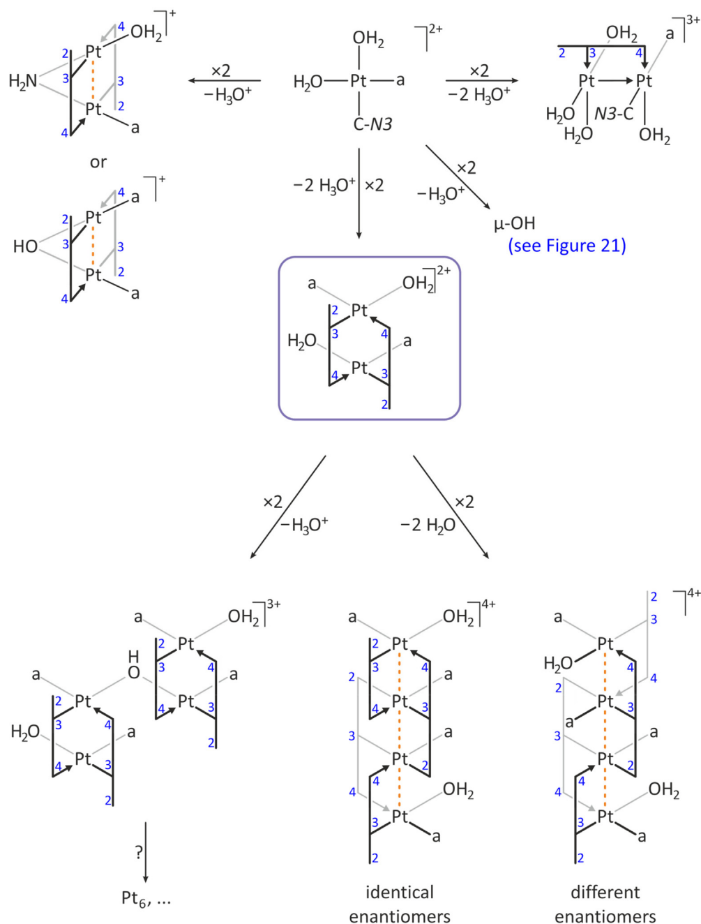
Fig. 20. Proposal for possible condensation patterns of mononuclear cis - [Pt(NH_3)(1MeC-N3)(H_2O)_2]^{2+} and its head-tail dimer.
