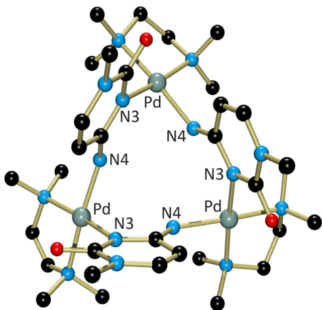
Fig. 15. View of the \text{C}_3 symmetric cation \{[(\text{tmeda})\text{Pd}(1\text{MeC}_{-H}\text{-N3,N4})]_3\}^{3+} [143].
