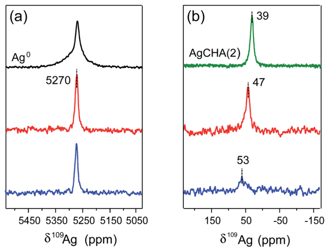
Fig. 7 109 Ag MAS NMR spectra in the regions of Ag 0 (a) and Ag + (b) of the AgCHA(2)-R-Ox (blue) and AgRHO(4)-R-Ox (red) zeolites. Ag metal (black) and AgCHA(2) (green) are the references for Ag 0 and Ag + , respectively.
