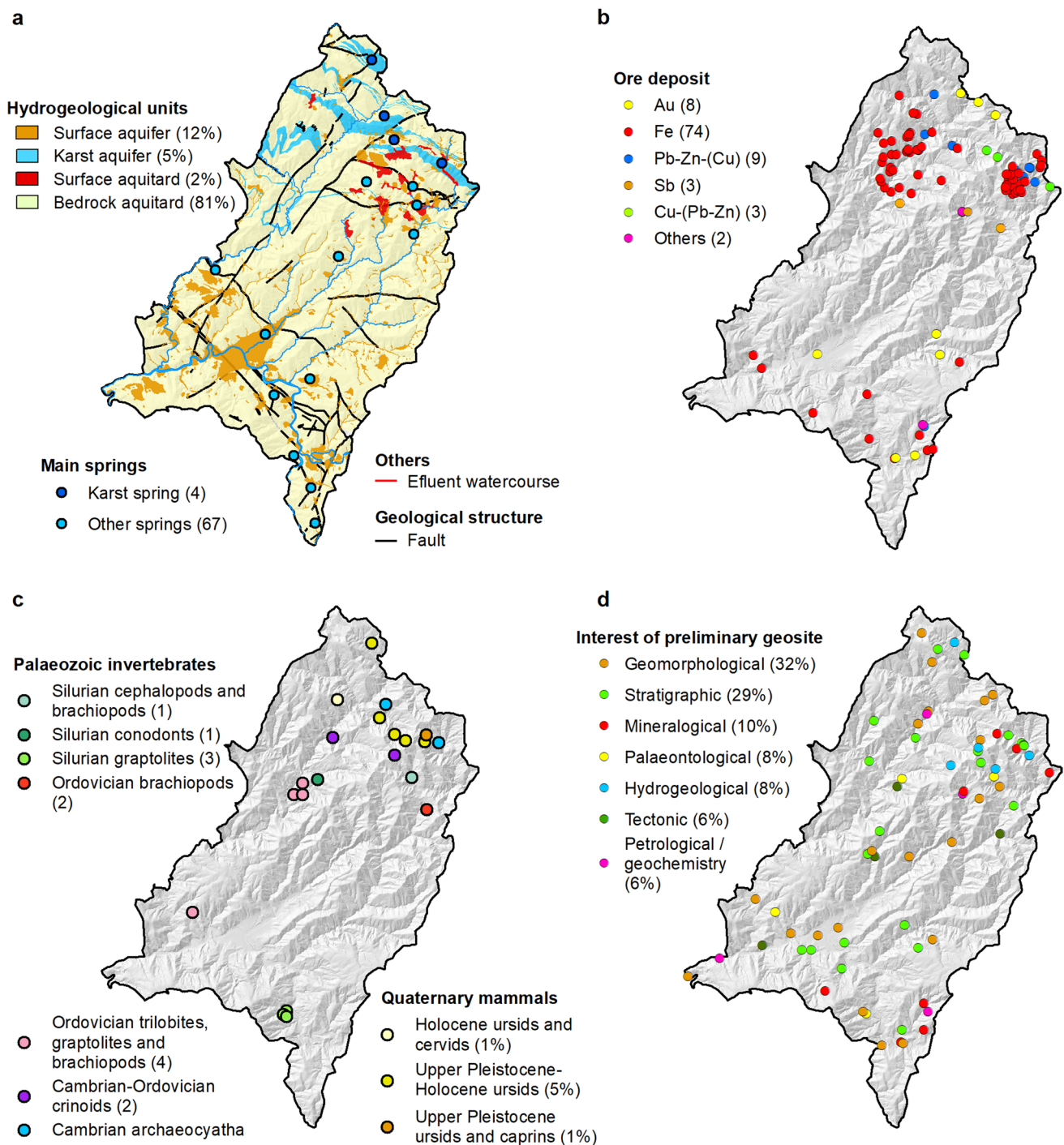
Fig. 6 Hydrogeology, metallogeny, palaeontology and geoheritage of the Courel Mountains UGGp. a Hydrogeological map depicting aquitards, aquifers, springs and an efluent watercourse. b Metallogenic map showing metallic ore deposits of economic interest. c Palaeontological
