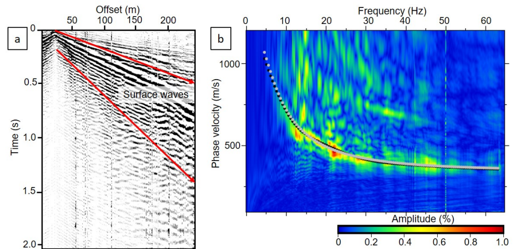
Figure 5. (a) Example seismic shot record with labelled red arrows showing the extent of the surface waves. (b) Corresponding dispersion diagram. The high amplitudes are indicative of the different phases (frequency and phase-velocity). The theoretical and inverted curves are shown as white and black dots, respectively.
