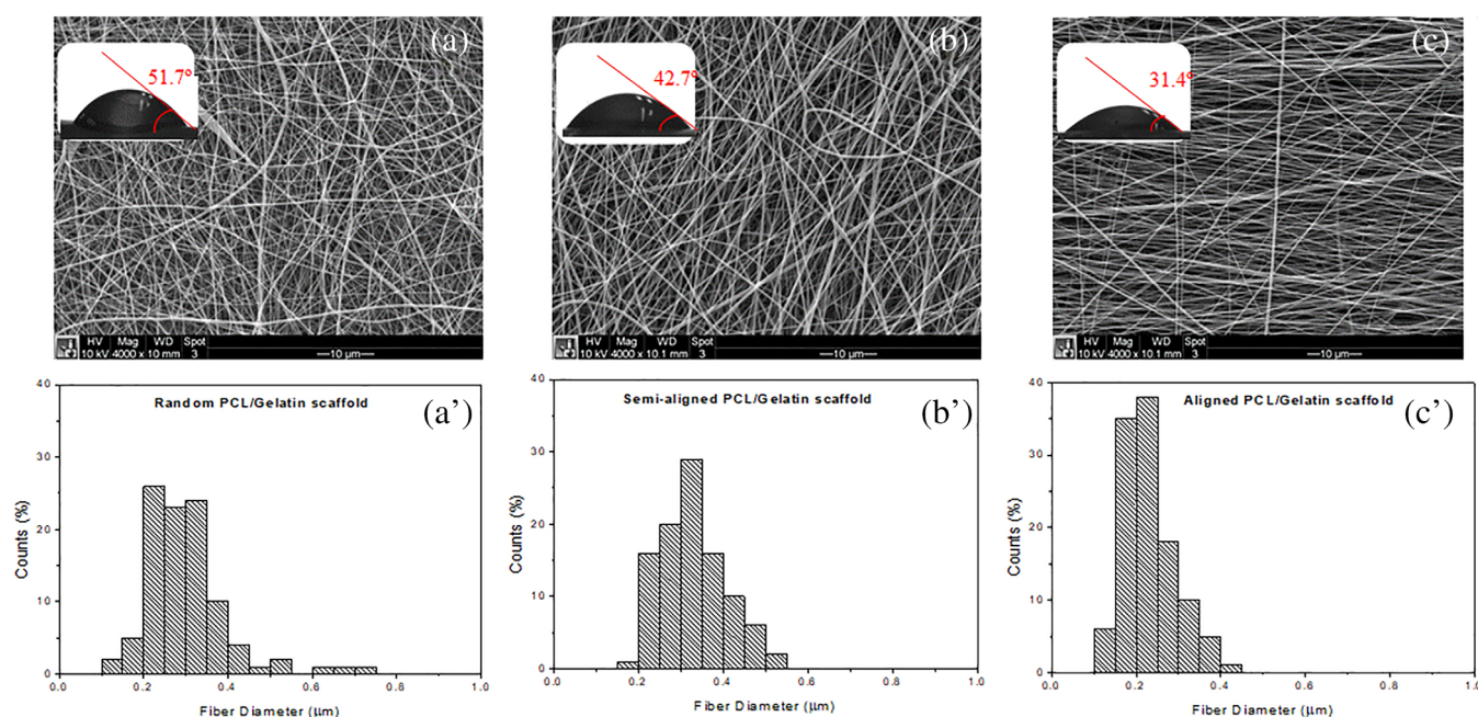
FIGURE 1 Contact Angle, scanning electron microscopy (SEM) images of the polycaprolactone (PCL)/gelatin scaffolds with different fiber alignments: (a) random, (b) semi-aligned and (c) aligned; fiber size distribution of the PCL/gelatin scaffolds with different alignments: (a') random, (b') semi-aligned and (c') aligned
