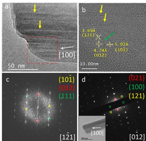
Figure 4. HRTEM analysis for two \pi -TiP_0 nanorods. (a) HRTEM micrograph for part of a rod. The yellow arrows show the stacking of the (012) planes along the long axis of the nanorod. The white arrow shows the direction [100] that make an angle of less than 10° with the direction of growth of the nanorod; (b) HRTEM micrograph for the area labelled by the red dashed square in (a) showing the presence of planar defects (indicated by yellow arrows) and the only area in the view (indicated by green arrow) where details in three directions can be visualized and indexed; (c) FFT pattern of the micrograph depicted in (b) showing the streaking of the diffraction spots corresponding to (012) plane seen along the zone axis [1-21]; (d) SAED pattern for another \pi -TiP_0 nanorod, shown in the inset, illustrating the streaking in the diffraction spots corresponding to the plane (021) seen along the zone axis [0-12].
