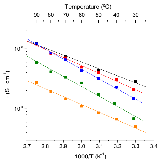
Figure 7. Plot of measured proton conductivity as function of temperature (Arrhenius plot) for \pi\text{-TiP}_x series at 95%-RH: as-synthesized \pi\text{-TiP}_0 (black), water-leached \pi\text{-TiP}_4 (red) and \pi\text{-TiP}_{10} (green), partially rehydrated \pi\text{-TiP}_{10} (orange) and \text{H}_3\text{PO}_4@ \pi\text{-TiP}_{10} (blue).
