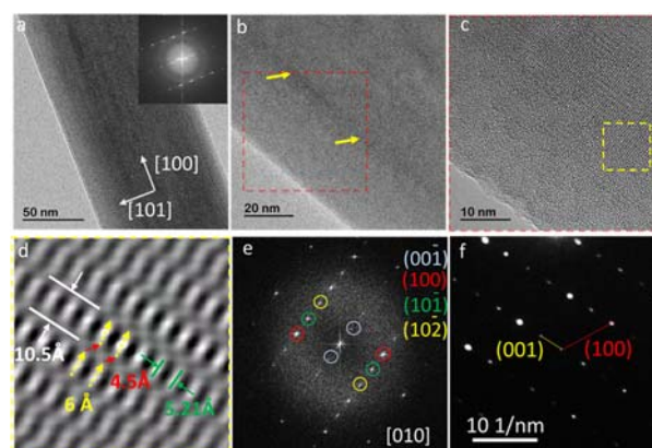
Figure 3. HRTEM analysis for a nanorod of \pi -TiP 0 . (a) TEM micrograph for a part of the \pi -TiP 0 nanorod and the inset is its FFT. The white arrows indicate the directions [100] and [101]; (b) A magnification of the nanorod in (a) showing the crystal imperfections indicated with yellow arrows; (c) HRTEM micrograph for the area indicated by the dashed red square in (b); (d) A processed HRTEM image for the area enclosed by the dashed yellow square in (c) showing the direction of the stacking faults; (e) FFT pattern for (c) and its indexing showing the streaking of the reflection spots corresponding to plane (00-1) seen along the zone axis [010]; (f) SAED pattern of the nanorod shown in (a) taken in the same zone axis [010] showing the streaking of the diffraction spots of (001) plane.
