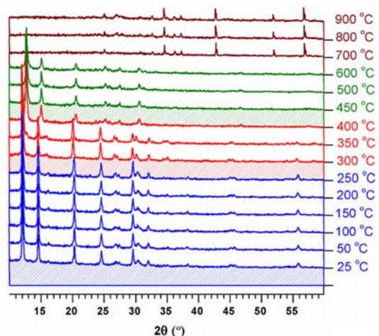
Figure 5. HT-PXRD pattern of \pi -TiP_0 recorded heating up from 25 °C to 900 °C in an open air. Color codes correspond to the structural changes: blue – pristine \pi -TiP_0 phase, red – partially dehydrated \pi -TiP, green – completely dehydrated \pi -TiP, brown – a mixture of TiP 2 O 7 , Ti 5 O 4 (PO 4 ) 4 phases.
