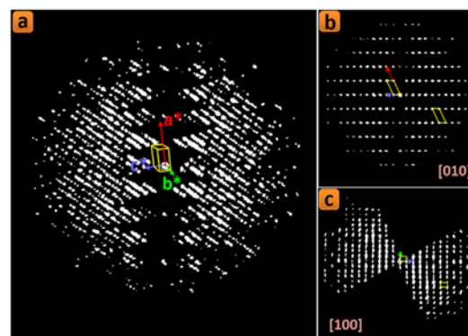
Figure 2. (a) The 3D reconstruction of the reciprocal space from an electron diffraction tilt series of a single \pi -TiP 0 nanorod with ADT3D software (b) and (c) The projection of the 3D reciprocal space along the zone axes [010] and [100], respectively.
