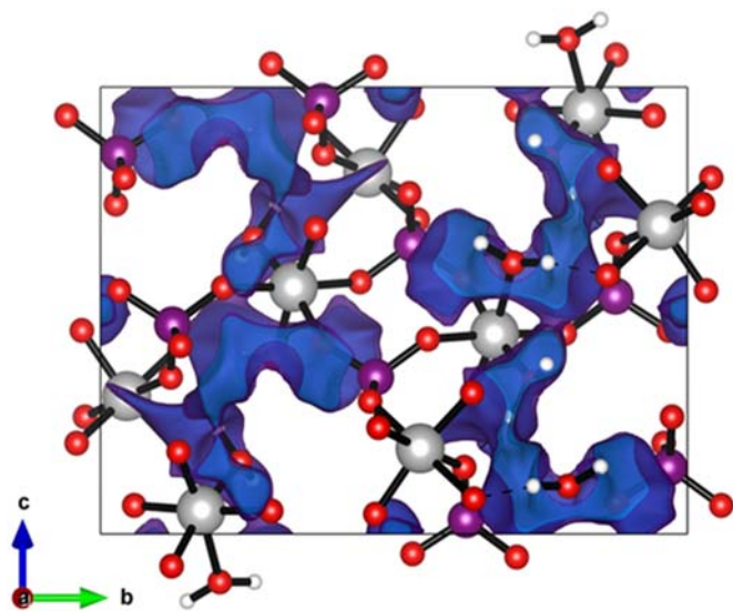
Figure 8. Projection of bond valence energy landscape calculated for onto ( bc ) plane. Darker colours are assigned for inner isosurface levels ( > 0.7 \text{ eV} ) while the lighter hues indicate the outer levels ( < 0.65 \text{ eV} ).
