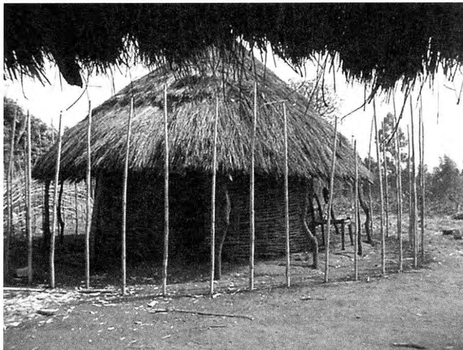
Fig. 7: Building an external ring to enlarge a kitchen and transforming it in a main house. Gundul (Asosa).
