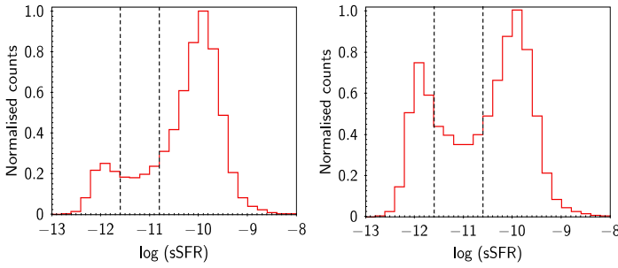
Figure 2. Distributions of sSFR for UV (left panel) and optical (right panel) samples. Green valley region is represented in between the two black dashed lines.
