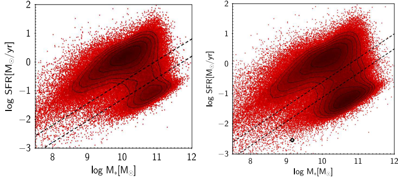
Figure 3. SFR versus stellar mass for UV sample (left panel) and optical sample (right panel). Green valley region is represented in between the two black dashed lines.
