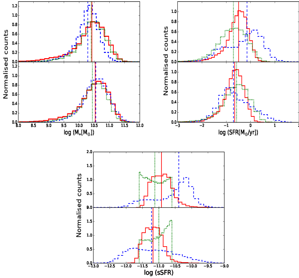
Figure 4. Comparison of stellar mass, SFR, and sSFR in optical (top panels) and UV (bottom panels). The blue dashed, green dotted, and red solid histograms in all figures represent the green valley sample selected using colours ( M_{NUV}-M_r and M_g-M_r ), sSFR, SFR vs. stellar mass criterion. The vertical dashed lines in all figures represent the median values for each histogram, where each median has the same colour as the one of the corresponding histogram.
