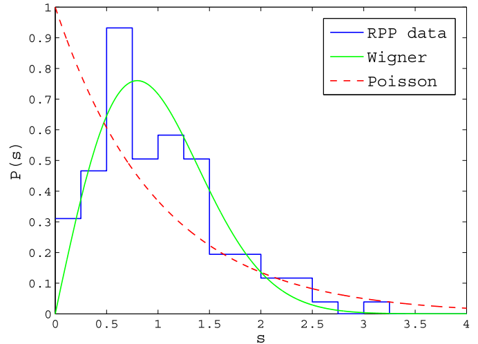
Fig. 1. (Color online.) NNSD for the experimental spectrum (histogram) from the RPP, compared to the Wigner surmise (solid) and the Poisson distribution (dashed).
