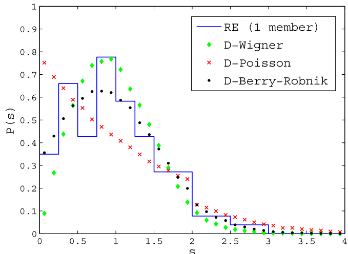
Fig. 5. (Color online.) NNSD for one single realization of the RE (histogram) compared to the distorted distributions: Wigner (D-Wigner, diamonds), Poisson (D-Poisson, crosses) and Berry–Robnik with f = 0.78 (D-Berry–Robnik, dots).
