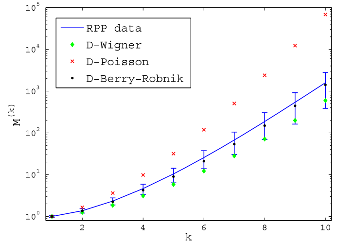
Fig. 3. (Color online.) Moments of the NNSD, M^{(k)} , for the experimental spectrum (solid line with error bars), from the RPP, compared to those of the distorted distributions: Wigner (diamonds), Poisson (crosses) and Berry-Robnik with f = 0.78 (dots).
