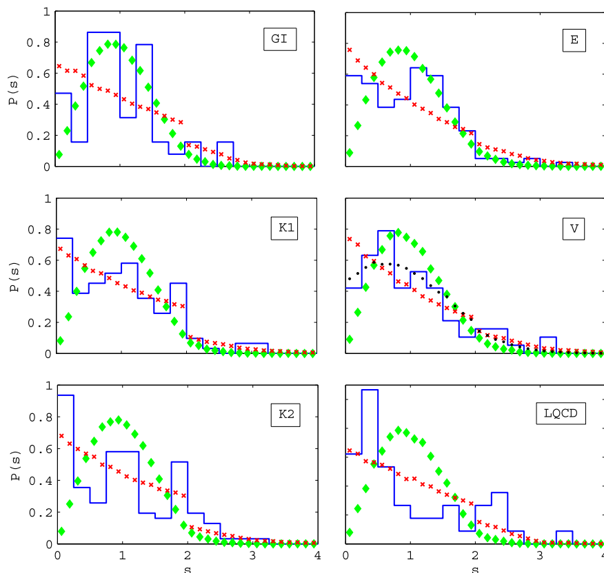
Fig. 6. (Color online.) NNSDs for the theoretical spectra: (i) top left, set GI by Godfrey and Isgur [14]; (ii) middle left, set K1 by Koll et al. [11]; (iii) bottom left, set K2 by Koll et al. [11]; (iv) top right, set E by Ebert et al. [13]; (v) middle right, set V by Vijande et al. [12] and ad hoc distorted Berry–Robnik with f = 0.63 ; (vi) bottom right, set LQCD by Dudek et al. [16]. Distorted Wigner (D-Wigner) is represented with diamonds, distorted Poisson (D-Poisson) with crosses and distorted Berry–Robnik (D-Berry–Robnik) with dots.
