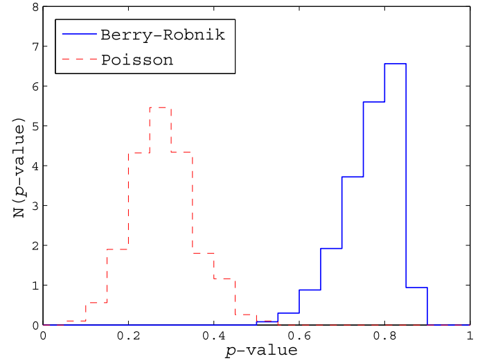
Fig. 4. (Color online.) Distributions of the p -values of the K-S test for the 1000 “realizations” of the experimental spectrum within the error bars, for the null hypothesis that the distribution coincides with Poisson (dashed histogram) and with Berry-Robnik for f = 0.78 (solid histogram).
