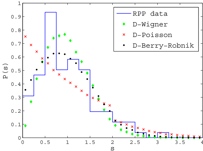
Fig. 2. (Color online.) NNSD for the experimental spectrum (histogram) from the RPP, compared to the distorted distributions: Wigner (D-Wigner, diamonds), Poisson (D-Poisson, crosses) and Berry-Robnik with f = 0.78 (D-Berry-Robnik, dots).
