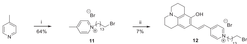
Scheme 3. Synthesis of compound 12 . Reagents and conditions: (i) Br-(CH 2 ) 14 -Br, CH 3 CN, 48 h; (ii) 9-Formyl-8-hydroxyjulolidine, piperidine, 75 °C, 24 h.
