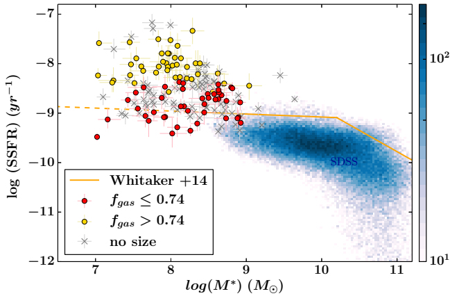
Fig. 12. Diagram of sSFR vs. M_* for our galaxies, coded by f_{\text{gas}} (below). The segregation is evident between galaxies with higher and lower gas fraction than the median f_{\text{gas,med}} = 0.74 . The EELG fraction is evidenced with yellow colored circles.
