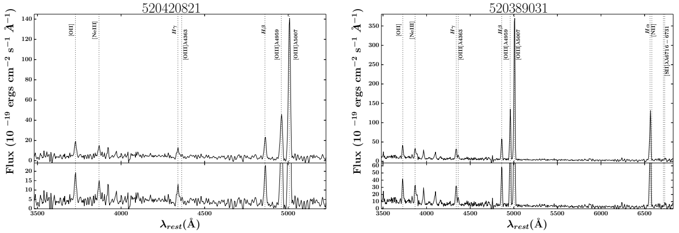
Fig. 2. Observed spectra of two galaxies in VUDS with strong emission lines and faint continuum. The galaxy on the left and right hand side panels are at redshift z = 0.555 and z = 0.173 , respectively. While for the former the H\alpha line lies outside the wavelength range, for the latter it is still visible in the red part of the spectrum. Dotted lines and labels indicate some of the relevant emission lines detected.
