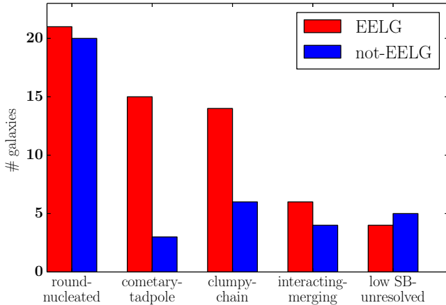
Fig. 7. Bar histogram showing the number of galaxies falling into each morphological class described in the text for EELG (red) and non-EELG (blue) subsamples. We find that EELGs have a higher fraction of irregular and disturbed morphologies (58%) compared to non-EELGs (34%). Only galaxies in COSMOS and ECDFS fields are considered for this analysis.
