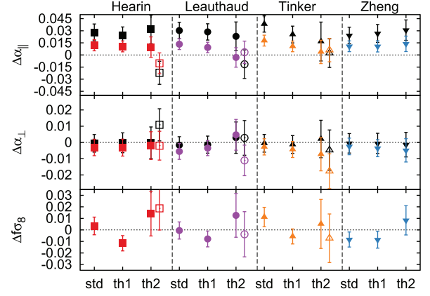
Figure 11. Inferred scaling parameters, \alpha_{\parallel} and \alpha_{\perp} , and f\sigma_8 using a BAO (black symbols) and FS (coloured symbols) type of analysis from the pre-reconstructed OUTERIM-HOD mocks, for different types of HOD models and flavours (listed in the x-axis). Red, purple, orange, and blue colours correspond to Hearin, Leauthaud, Tinker and Zheng HOD models for the FS type of analysis, respectively. For each of these models three flavours have been implemented: standard (std), threshold 1 (th1), and threshold2 (th2), as labelled. The filled symbols correspond to 1 h^{-1}\text{Gpc} -size cubic box without periodic boundary conditions. The empty symbols correspond to the results obtained from a padded and larger box corresponding to 3 h^{-1}\text{Gpc} -size, where the non-periodicity impact is negligible. All results correspond to fitting the mean of 27 mocks, and the reported error is 1\sigma of the error of the mean.
