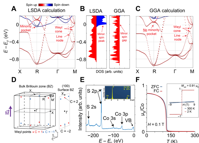
Fig. 1. Electronic structure and characterization of CoS 2 samples. (A) Band structure obtained from LSDA. (B) Comparison of DOS from both spin channels for LSDA and GGA. The red solid area shows the majority spin, and the blue solid area shows the minority spins. (C) Band structure obtained from GGA. (D) Illustration of the Weyl points in the bulk Brillouin zone, which are located on the high symmetry planes k_x = 0 and k_y = 0 parallel to the magnetization direction \vec{M} . Red dots indicate Weyl points with positive Chern number C ; blue dots indicate Weyl points with negative Chern number. (E) Core-level spectroscopy measured with photon energy h\nu = 602 eV; arrows indicate elemental core levels and valence band (VB). Inset shows energy-dispersive x-ray spectroscopy (EDX) curves, showing an ideal stoichiometry. (F) Temperature dependence of magnetization curve under zero field-cooling (ZFC) and field-cooled (FC) conditions; the applied field is 0.1 T. The Curie point at 130 K is indicated. The inset shows the magnetic field dependence below and above the Curie temperature. The measurements were taken along the [100] direction.
