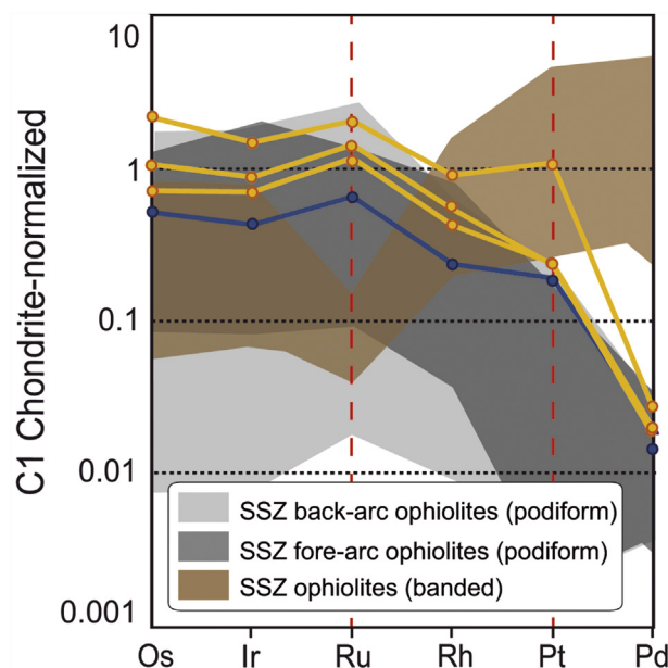
Fig. 6. C1 chondrite-normalized (Naldrett and Duke, 1980) patterns of Loma Caribe chromitites and comparison with other mantle-hosted chromitites. Data sources are Economou (1983), Pedersen et al. (1993), Melcher et al. (1997), Economou-Eliopoulos (2010), and Arai (2013), and references therein. Yellow symbols = chromitite pods; blue symbols = chromitite veins.
