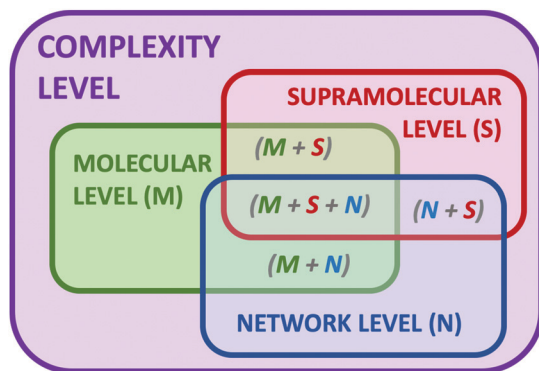
Fig. 1 Schematic representation of the different levels within chemical systems, connecting molecular (M), supramolecular (S) and network (N) levels. Complexity can be expressed at all levels, as well as through their corresponding combinations.
