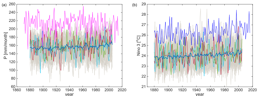
FIG. 14. Comparison of large-area averages in model (MPI-ESM) and observation (precipitation: AISMR, magenta; SST: ERSST v5, blue): (a) JJAS precipitation and (b) JJA SST. To match the AISMR data, precipitation in the model is averaged over the AISMR areas (India, except for a few states; see main text). The JJA SST is averaged over the Niño-3 box. Thin gray lines represent all converged members of the MPI-GE, while three colored lines show examples of individual members; the thick blue lines show the ensemble mean.
