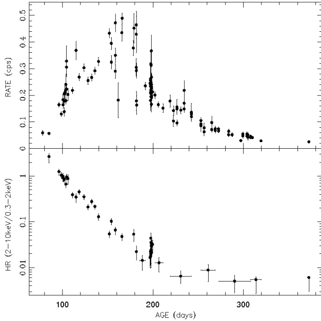
Figure 1. V1369 Cen x-ray (top panel) and hardness ratio (HR, bottom panel) light curves obtained from Swift -XRT observations.
