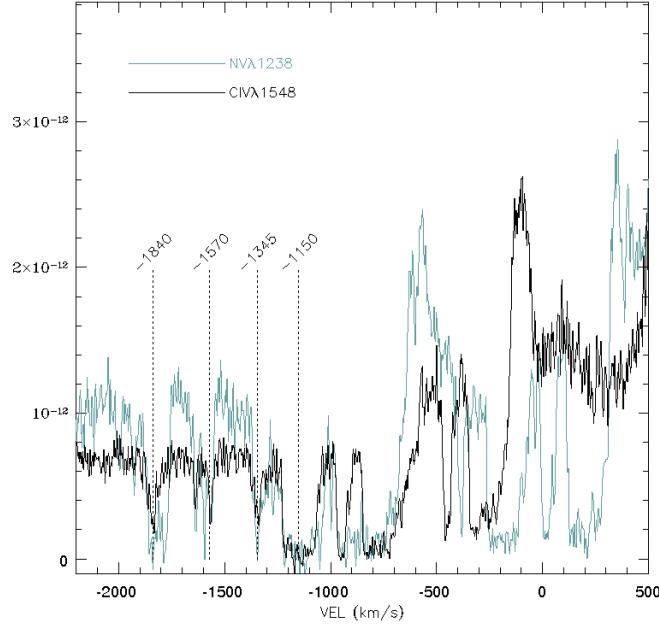
Figure 6. The absorption structures observed in the day 837 spectrum for the transitions NV\lambda\lambda 1238,1242\text{\AA} and CIV\lambda\lambda 1548,1550\text{\AA} . Vertical dotted lines mark the approximate wavelength of the absorption components used for the N/C ratio computation. The y-axis is flux in \text{ergs}/\text{cm}^2/\text{s}/\text{\AA} .
