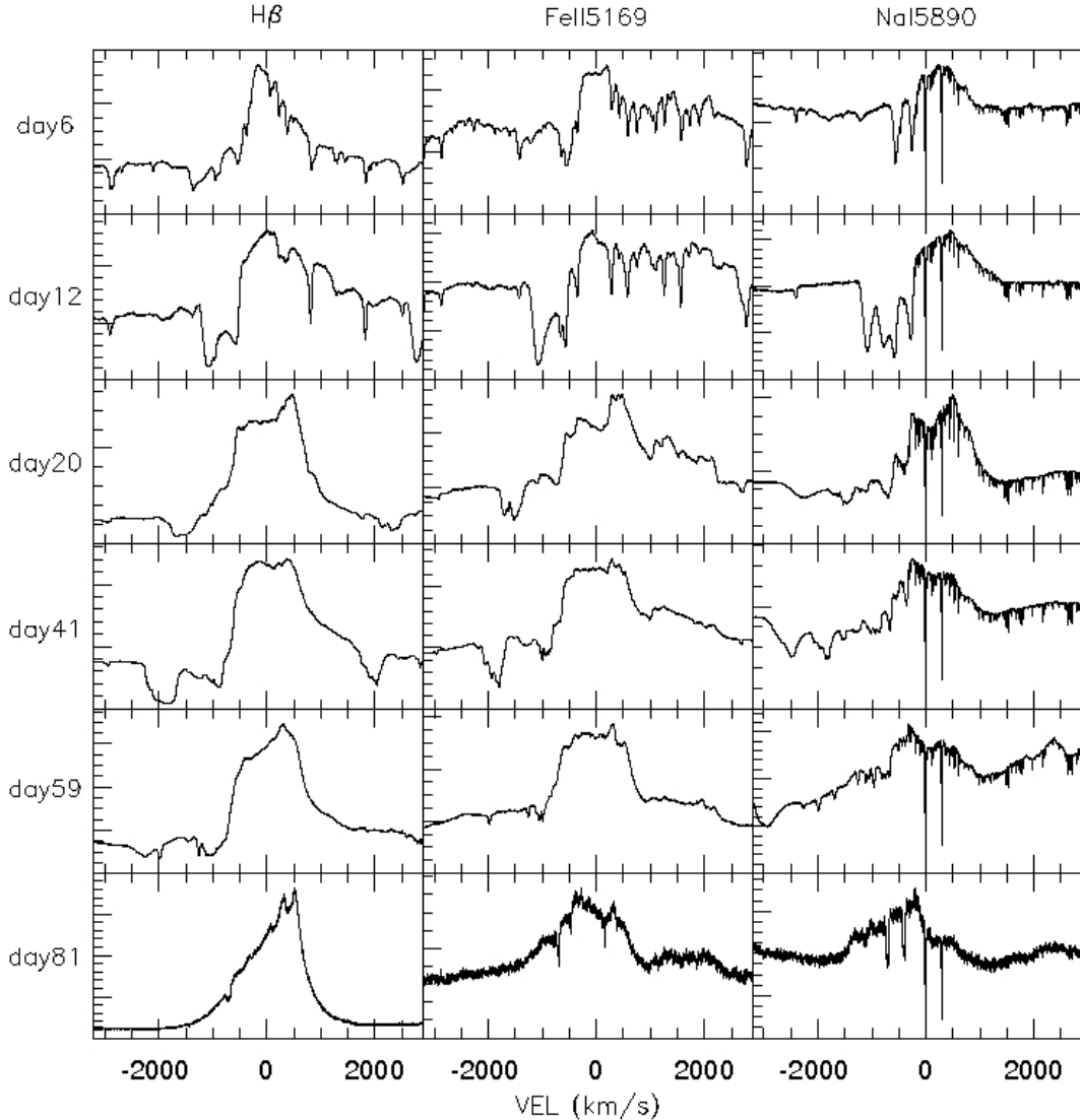
Figure 16. V1369 Cen early decline line profiles.
