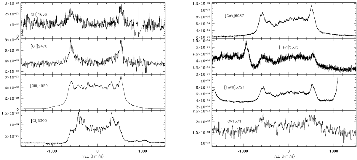
Figure 8. Line profiles of different ions in V1369 Cen spectrum of day 566. Left panel: intercombination and forbidden transition from low energy ions of oxygen (the ionization potential (IP) of \text{O}^{4+} is \sim 55\text{eV} ). Right panel: forbidden and recombination transitions from high energy ions: \text{IP}(\text{Ca}^{4+}) \sim 67\text{eV} , \text{IP}(\text{Fe}^{5+}) \sim 76\text{eV} , \text{IP}(\text{Fe}^{6+}) \sim 100\text{eV} , \text{IP}(\text{O}^{6+}) \sim 113\text{eV} .
