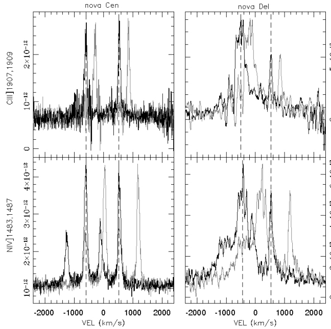
Figure 5. V1369 Cen (left) and V339 Del (right) CIII] (top) and NIV] (bottom) line profiles at their last epoch. The black color is for CIII] \lambda 1908\text{\AA} (NIV] \lambda 1486\text{\AA} ), while the gray is for CIII] \lambda 1906\text{\AA} (NIV] \lambda 1483\text{\AA} ). Vertical dashed lines mark the blue and red peaks of the emission line. V339 Del asymmetric profiles indicate geometrical (at the substructure level) asymmetry. Density inhomogeneity is also possible but cannot be verified from the lines themselves because the doublets are blending.
