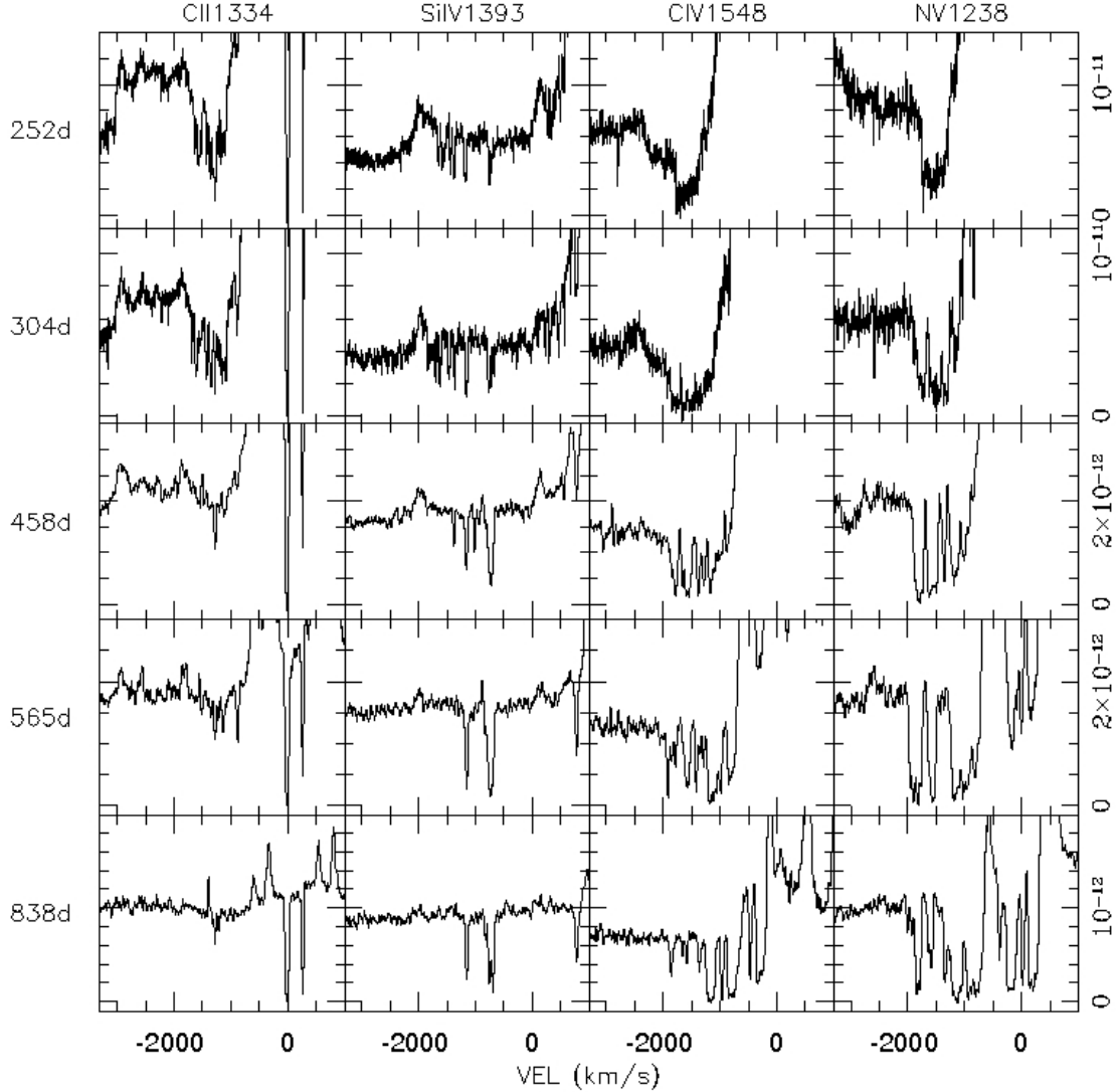
Figure 12. V1369 Cen ionization structure as evinced from the absorptions observed in the permitted resonant transitions. The transitions and the epoch of each observations are labeled on the figure side (top and left respectively). On the right axis of the plot, fluxes are in \text{erg}/\text{cm}^2/\text{s}/\text{\AA} .
