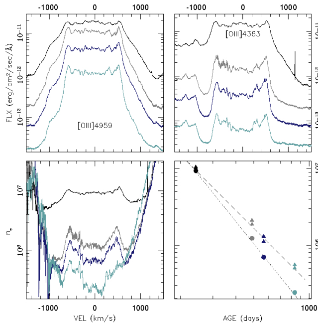
Figure 4. V1369 Cen [OIII] line profiles (top panels) and electron density as derived from the [OIII] emissions diagnostic: in velocity space at various epochs (bottom left panel) and as function of time (bottom right panel). Note that both fluxes (top two panels) and densities (bottom two panels) are in log scale to enhance the contrasts. Different color indicates different epoch as it can be evinced from the bottom right panel. In the bottom right panel solid circles indicate the average density as measured in the velocity interval -100 to 100 km/s, while the triangles indicates the average density at the two peaks centered at -600 and 500 km/s.
