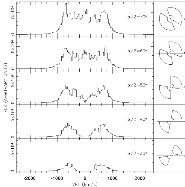
Figure 10. Line profiles produced by a biconical ejecta as simulated by Shore et al. (2013a). In all the cases it is assumed 1) an inclination of 40 deg of the observer with respect to the bi-cone axis, 2) an ejecta thickness of 0.7 \times R where, R is the maximum ejecta radius, and that the truncated cone is filled in. The simulation differs in the opening angle \alpha of the cone, indicated in the figure itself. A 2D sketch of the corresponding ejecta geometry is indicated on the right of each profile. The arrow points to the observer.
