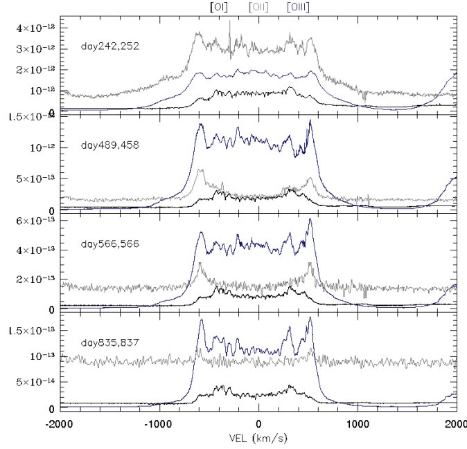
Figure 7. V1369 Cen ionization structure as evinced from the nebular lines [\text{OIII}]\lambda 4959\text{\AA} , [\text{OII}]\lambda 2470\text{\AA} and [\text{OI}]\lambda 6300\text{\AA} at the four epochs. Note that [\text{OIII}]\lambda 4959\text{\AA} has been scaled by a factor 0.1, while [\text{OII}]\lambda 2470\text{\AA} has been scaled by a factor 0.4.
