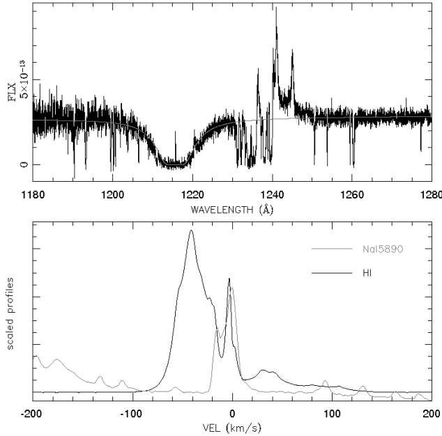
Figure 3. Top panel: Voigt profile fit of the Ly- \alpha interstellar absorption in the 837 day V1369 Cen spectrum. Bottom panel: comparison of the HI line profile from the GASS survey with the NaI interstellar absorption as seen against V1369 Cen’s maximum and early decline spectra. Note that the NaI absorption has been inverted for an easier comparison.
