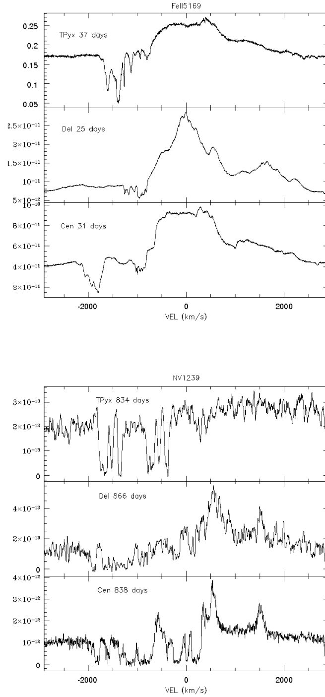
Figure 15. Absorption structures in the spectra of our “panchromatic novae” during early decline in the FeII \lambda 5169 \text{\AA} line (top), and during late nebular phase in the NV \lambda 1239 \text{\AA} transition (bottom).
