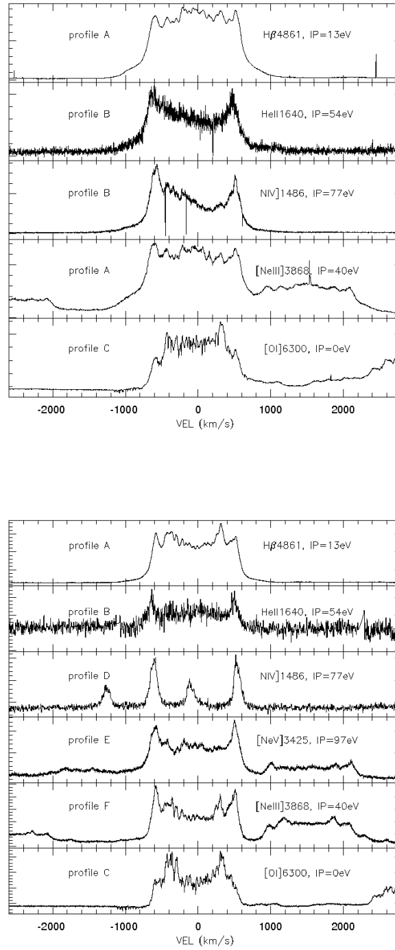
Figure 17. Master reference profiles used to aid the line identification in two illustrative epochs (top: day 252, bottom: day 836) of V1369 Cen spectral evolution.
