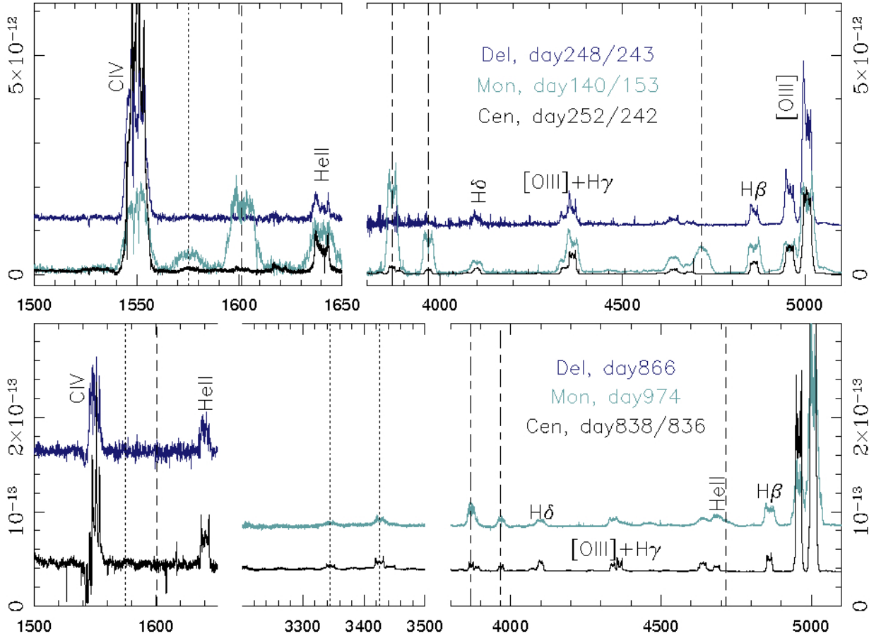
Figure 2. Comparison of V1369 Cen, V339 Del, and V959 Mon Ne emission lines at distinct epochs. Epochs and color-code identification of each spectrum is in the figure itself. The abscissa is in \text{\AA} and the ordinate in \text{erg/s/cm}^2/\text{\AA} . Note that top and bottom panels cover different wavelength ranges. All spectra, but V1369 Cen optical spectra of days 242 and 835, have been smoothed with a running boxcar filter of size in the range 5 to 19 points, depending on the S/N of the spectrum. The spectra have been scaled and shifted for an easier comparison: in the top panel, V339 Del has been shifted by the constant 1.1 \times 10^{-12} , V959 Mon has been scaled by a factor 10 and V1369 Cen has been scaled by a factor 1/18; in the bottom panel, V339 Del has been shifted by the constant 1.5 \times 10^{-13} , V339 Del has been scaled by the factor 20 and shifted by the constant 0.8 \times 10^{-13} , and V1369 Cen has been scaled by the factor 0.2. No spectrum has been corrected for reddening. The vertical lines mark the Ne transitions: the dotted line is for [NeV] \lambda 1575\text{\AA} and \lambda\lambda 3346, 3426\text{\AA} , dashed line is for [NeIV] \lambda 1602\text{\AA} and \lambda 4724\text{\AA} , while long and short dashed line is for [NeIII] \lambda\lambda 3869, 3968\text{\AA} .
