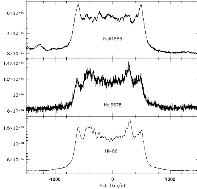
Figure 9. V1369 Cen H and He recombination line on day 835. On the y-axis of the plot, fluxes are in \text{erg}/\text{cm}^2/\text{s}/\text{\AA} .
