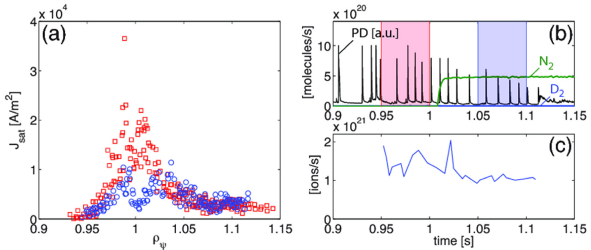
Figure 8. Effect of nitrogen seeding on inter-ELM outer-target saturation-current profiles: (a) ion-saturation profiles from LPs in intervals before and after seeding; (b) \text{D}_{\alpha} photodiode signal and nitrogen and deuterium injection rates; (c) integrated ion flux to outer target. Reproduced with permission from [77].
