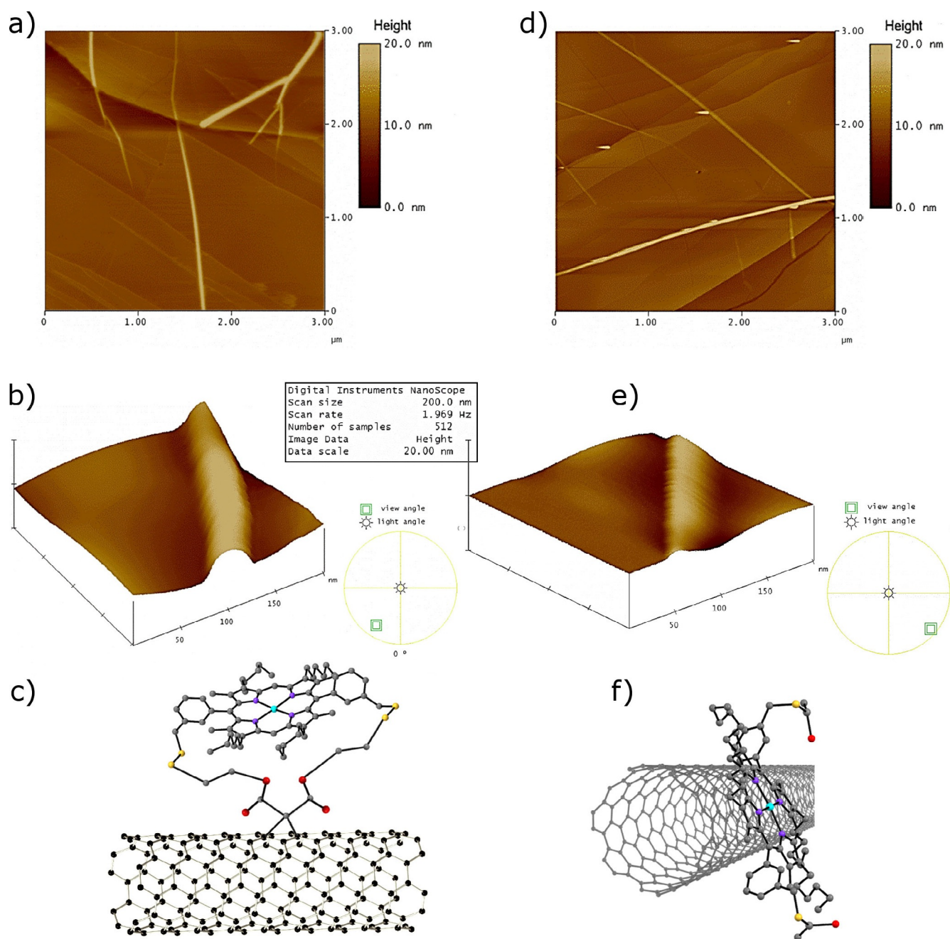
Figure 5. TM AFM imaging on mica surfaces. a, b) Image and 3D representation of AFM image of covalent Zn II -porphyrin@SWNTs nanohybrids ( 6 ). c) Schematic diagram of compound 6 ; d, e) Image and 3D representation of non-covalent Zn II -porphyrin@SWNTs nanohybrids ( 2 ). f) Schematic diagram of compound 2 .
