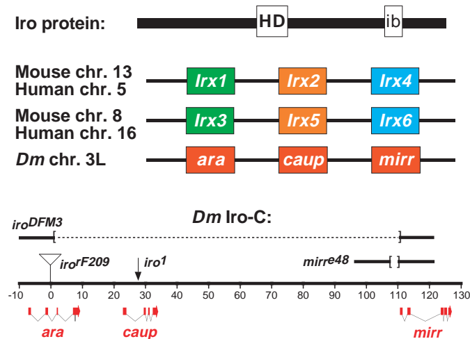
Fig. 1. Iro proteins and genomic organization of the Iro genes. All Iro proteins conform to the same structure with two strongly conserved domains: a homeodomain of the TALE class (HD) and the Iro box (ib), a motif reminiscent of the central part of the EGF repeats of the Notch receptor protein. Generally, Iro genes are chromosomally arranged in groups of three genes. Vertebrates paralogous genes are labelled with similar colours. A detailed physical map of the D. melanogaster ( Dm ) Iro-C is shown at the bottom of the figure. Molecular lesions associated with iro1 (chromosomal breakpoint), iroF209 (P element insertion), and iroDFM3 and mirre48 (chromosomal deletions) are indicated. Transcription units of the three Drosophila genes are shown in red. Coordinates are in kb. (Data taken from Bosse et al., 2000; Gómez-Skarmeta et al., 1996; McNeill et al., 1997; Netter et al., 1998; Peters et al., 2000.)
