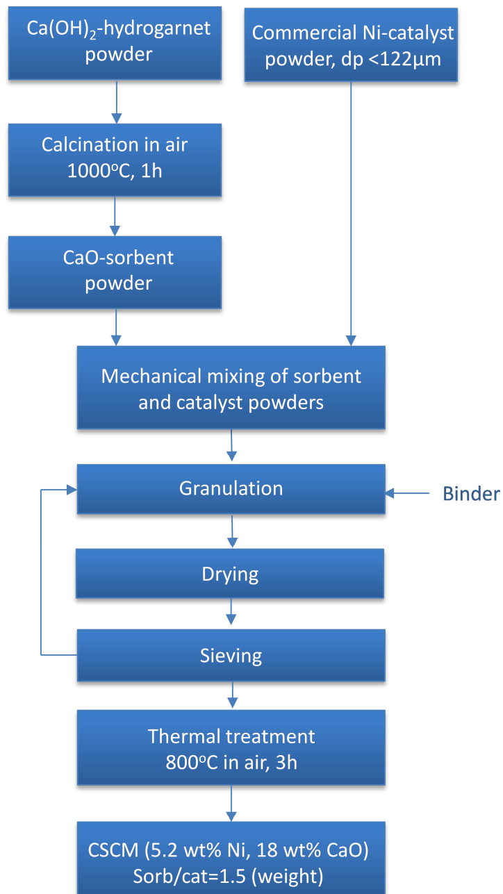
Figure S3: Scheme for preparation of CSCM by mechanical mixing of sorbent and catalyst powder followed by agglomeration and calcination
