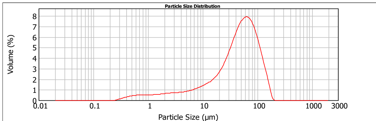
Figure S1: Particle size distribution of catalyst used in this work for CSCM production
